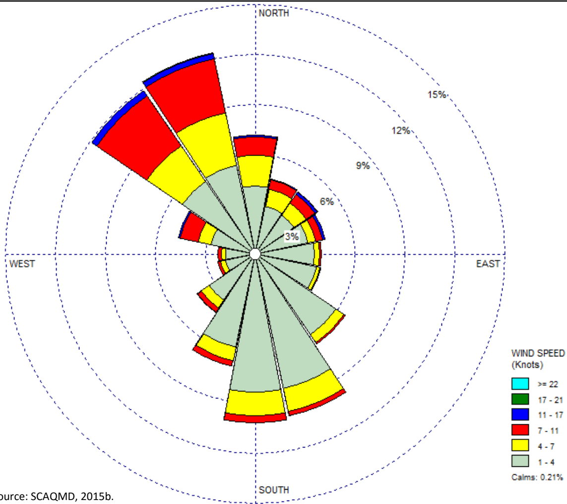
Figure C.4-1 – Wind Rose from Perris Valley Monitoring Station (2007 – 2011)
