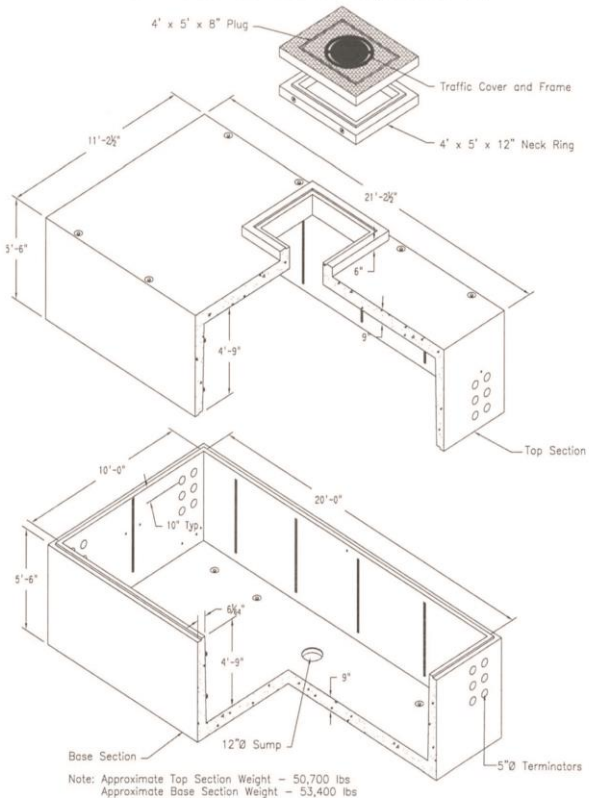
Figure D-7 Typical Subtransmission Vault
