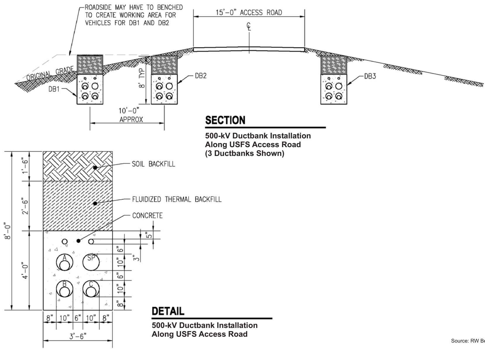
Figure B.4-4 Underground Transmission Cross-section in the ANF
