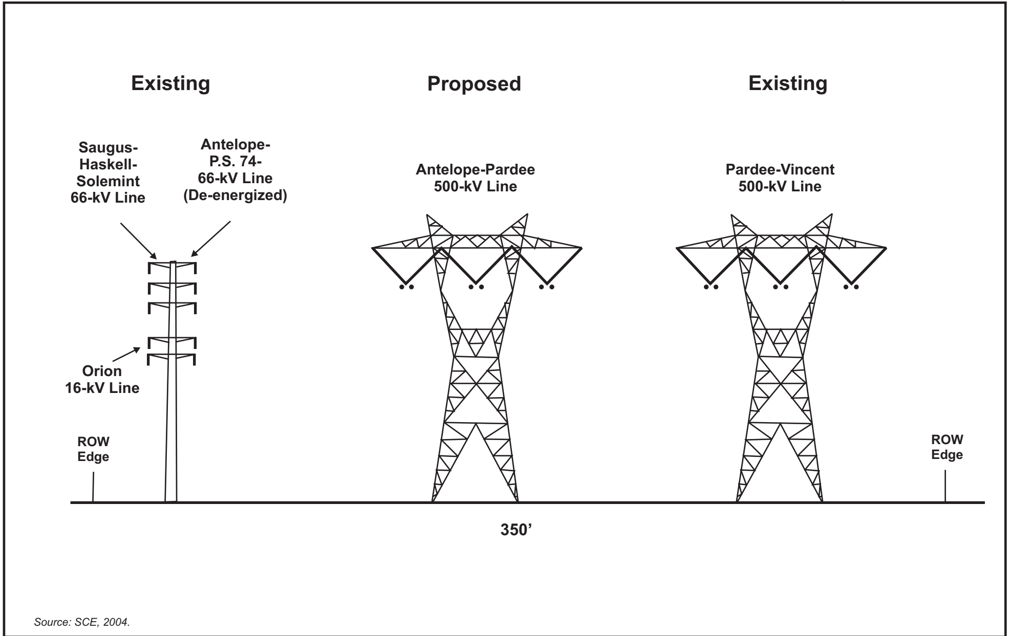
Figure B.4-11 Alternative 3 Proposed ROW Configuration For Mile 22.3 to Mile 25.6
