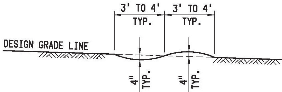
TYPICAL PROFILE
