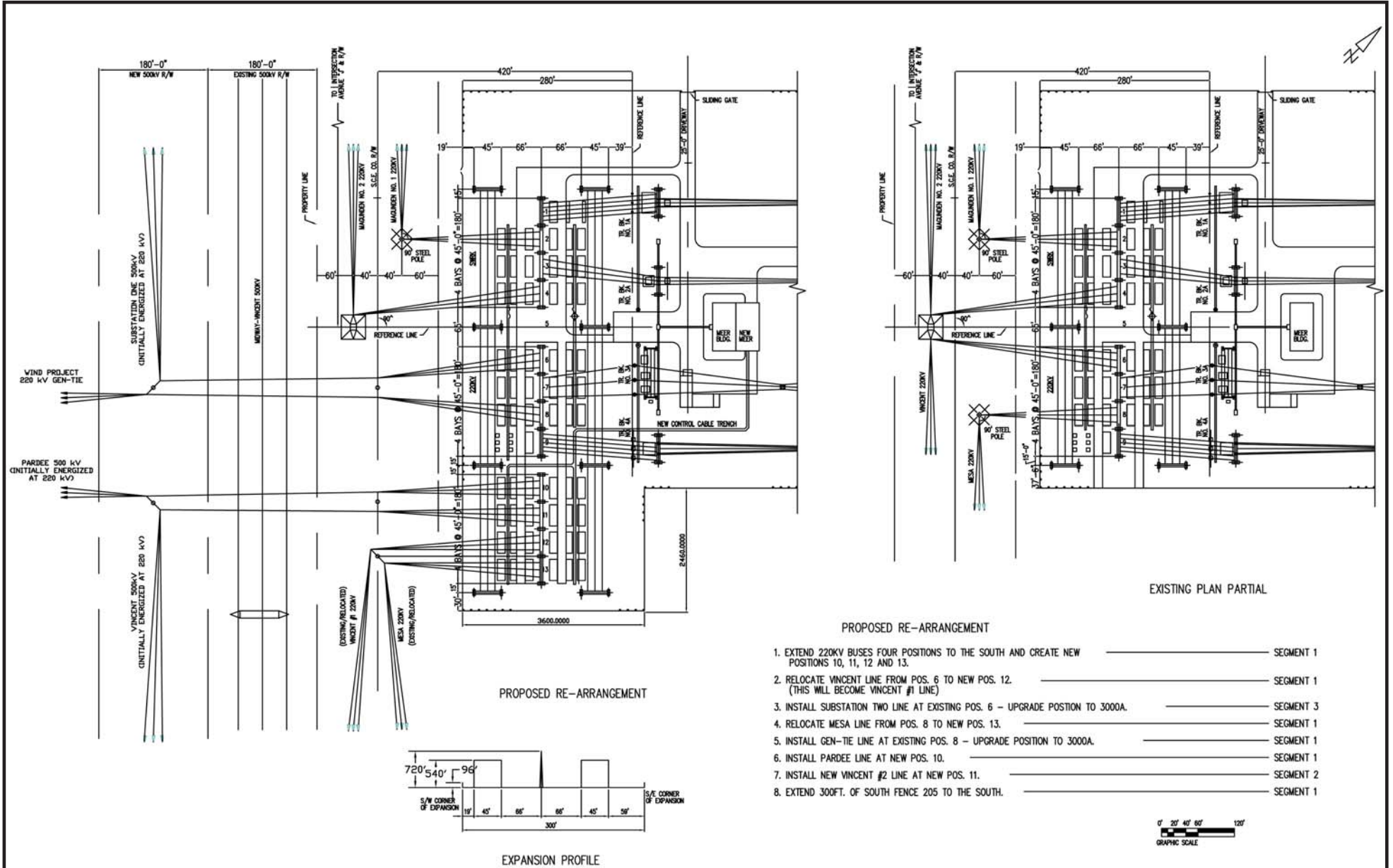
Figure B.2-28 Antelope Substation Plot Plan Detailing Proposed Modification
