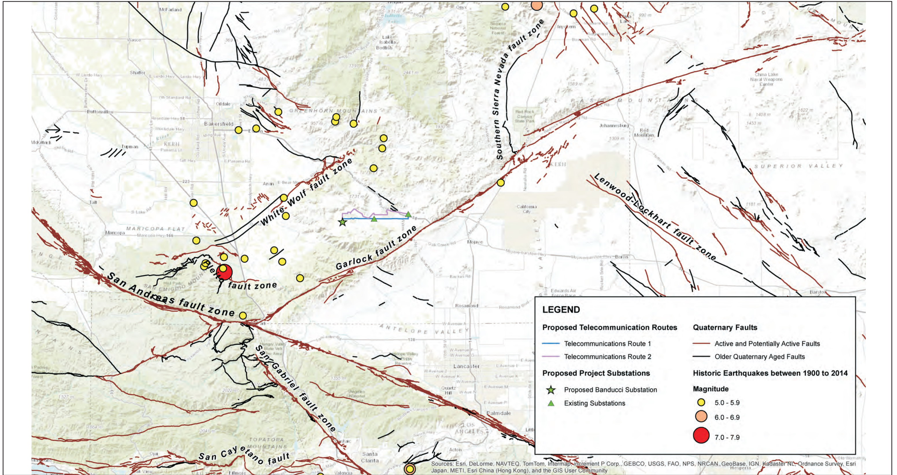
Figure 5.6-1 Regional Active Faults and Historic Earthquakes
