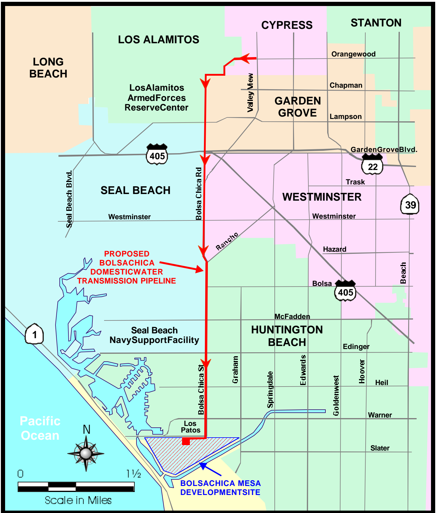
Proposed Route Bolsa Chica Domestic Water Transmission Line
