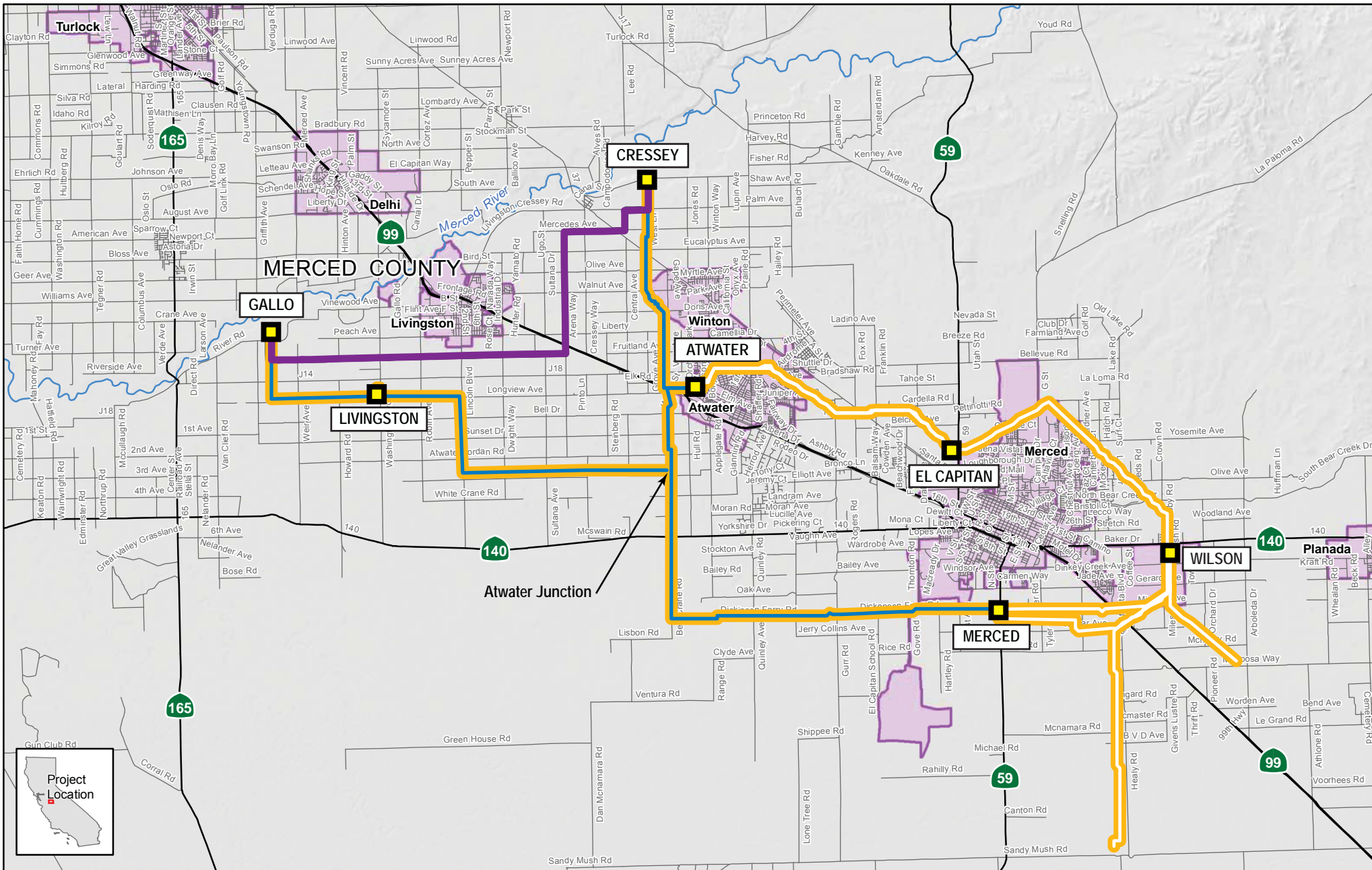
FIGURE 2.4-1 Existing Transmission System Cressey-Gallo 115 kV Power Line Project N 0 2 4 Scale: _____ Miles 1:200,000
