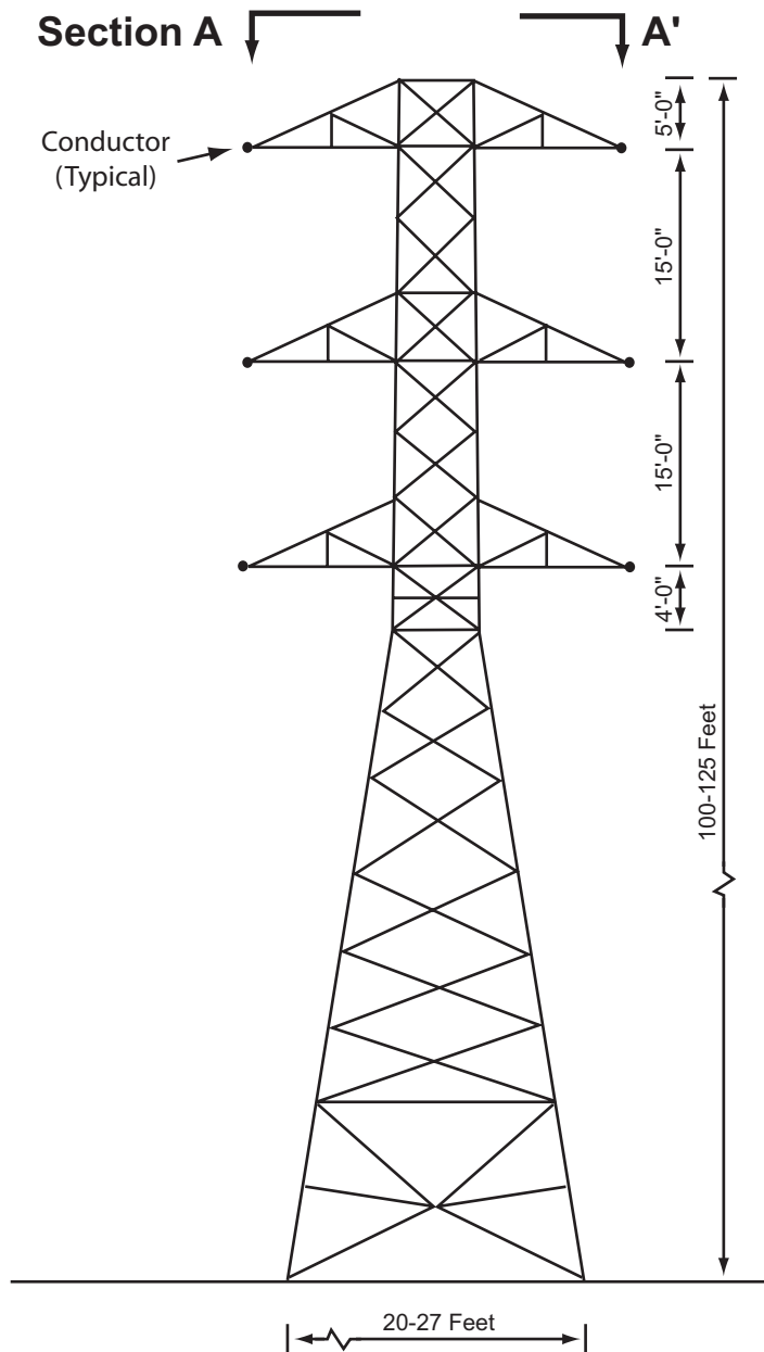
Profile View
