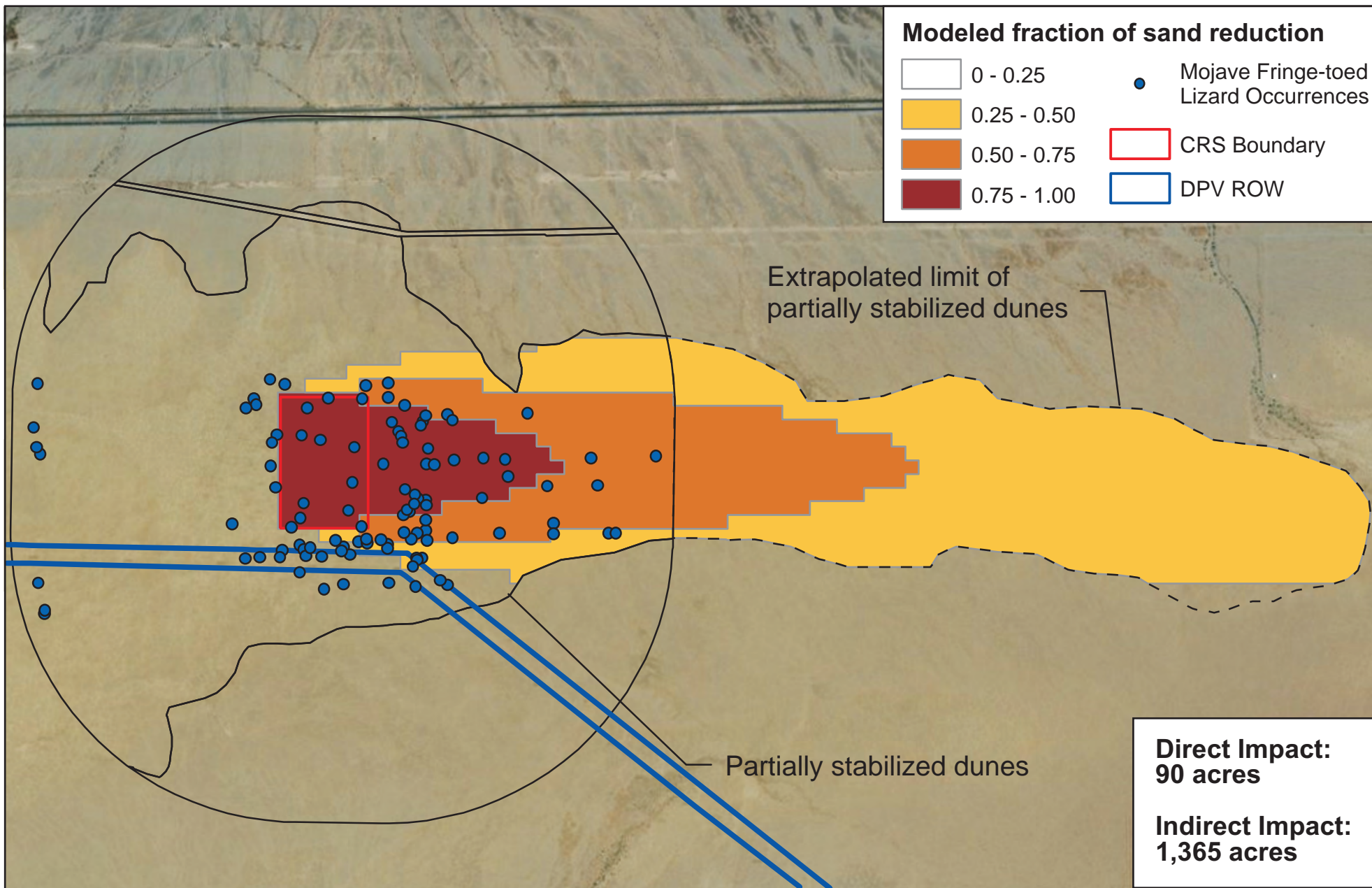
Figure D-2 MFTL Occurrences and Impacts – Proposed CRS Location
