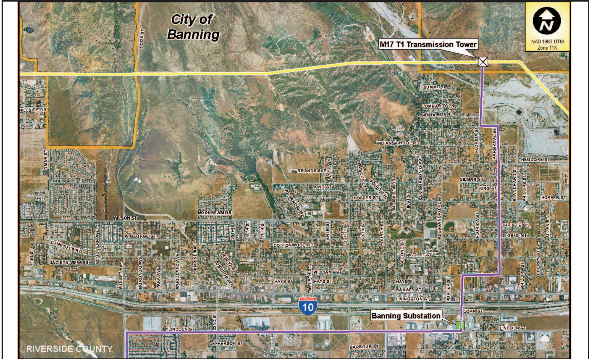
Figure B-15 Banning-M17 T1 Fiber Optic Cable Route
