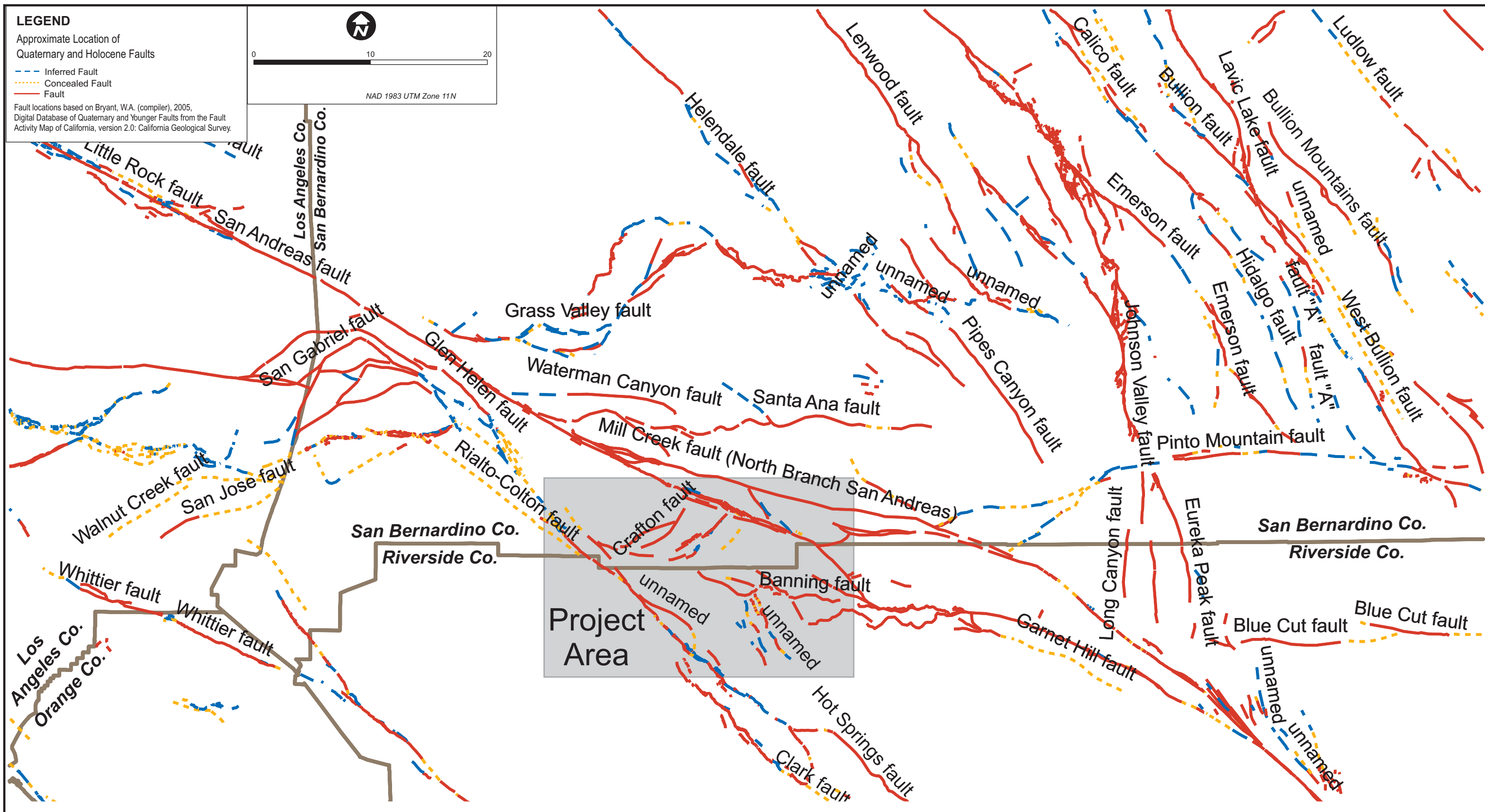
Figure D.6-1 Regional Fault Map
