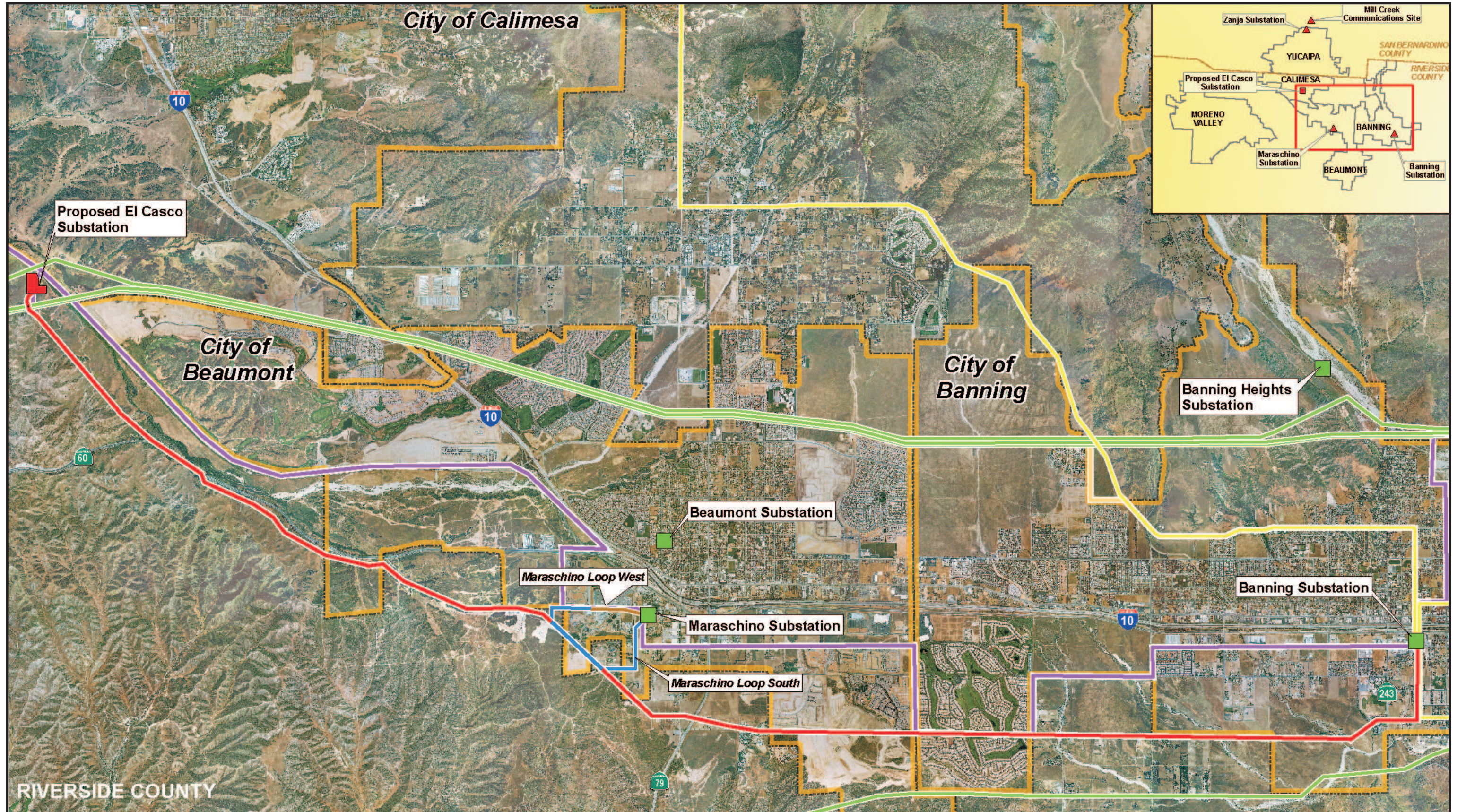
Figure B-2 Proposed El Casco Substation Site and 115 kV Subtransmission Line
