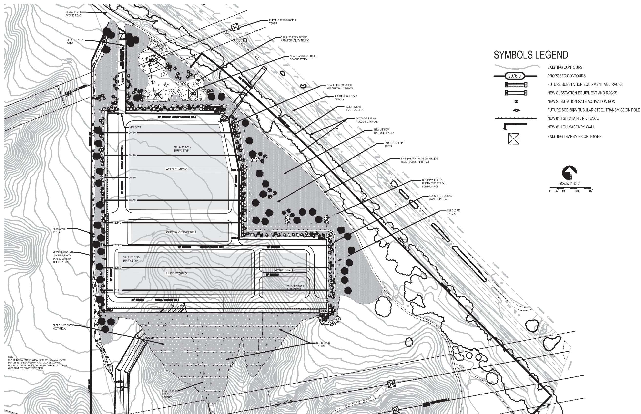
Figure B-3a El Casco Substation Site Plan
