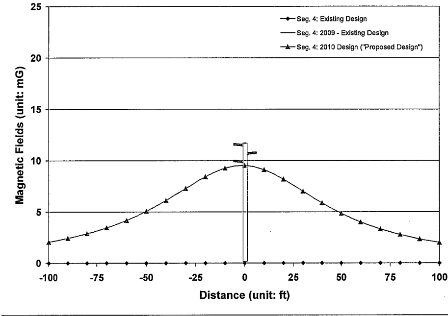
Figure 12. Magnetic Fields for Line Segment 4
