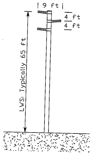
Figure 4. Proposed LWS Pole Single-Circuit 115 kV Design
