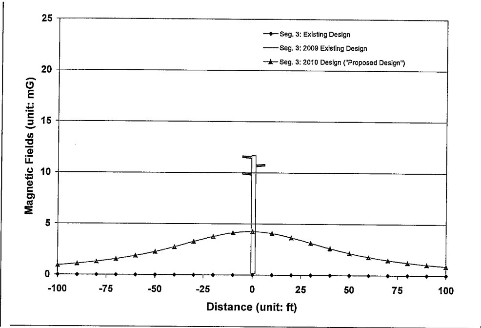
Figure 11. Magnetic Fields for Line Segment 3
