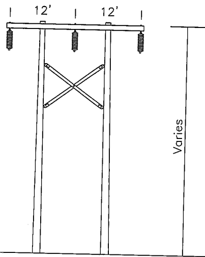
Figure 5. Existing 115 kV "H-Frame" Structure 26
