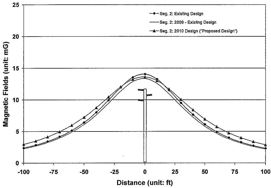
Figure 10. Magnetic Fields for Line Segment 2
