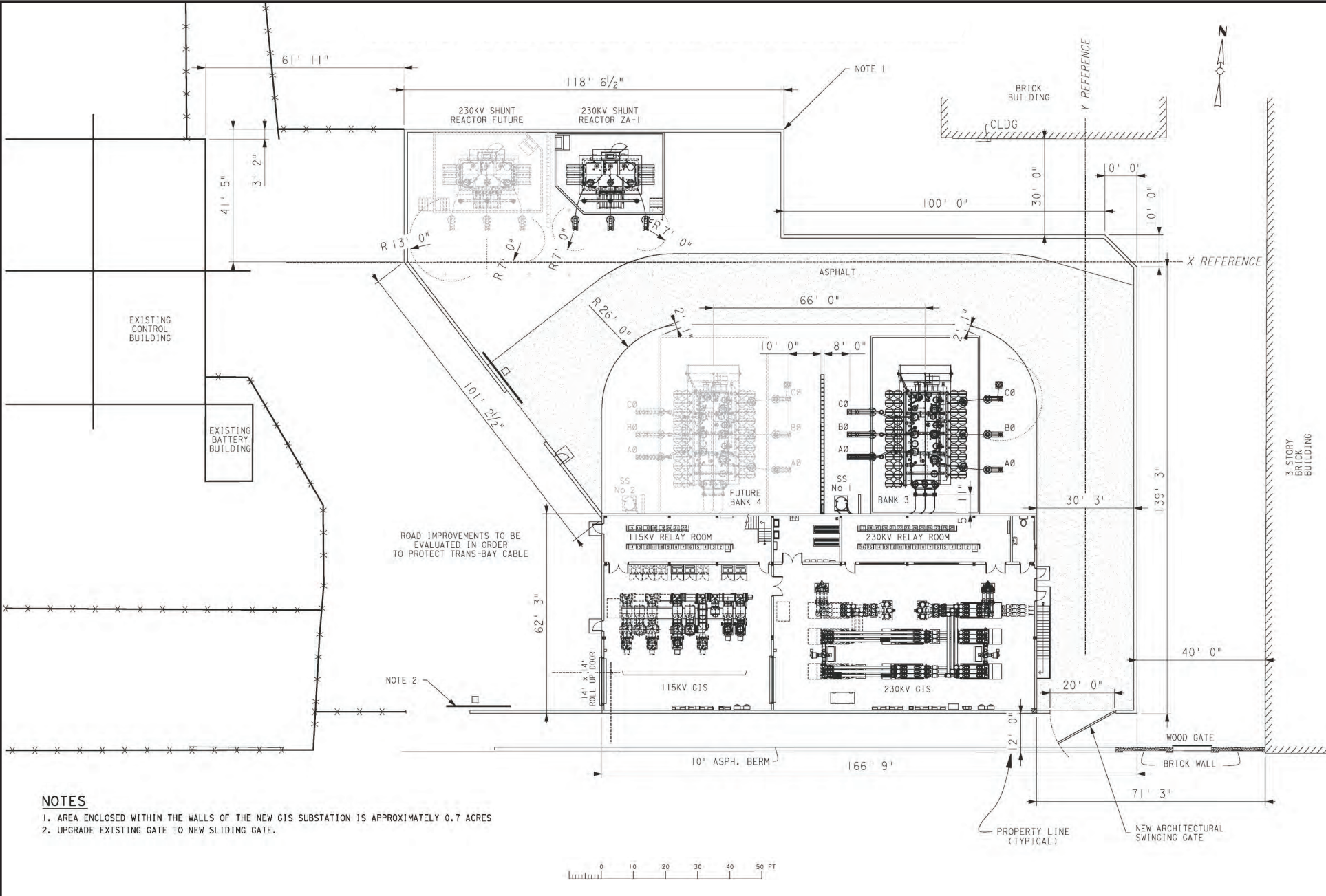
Figure 4-14a Revised Site Plan for Proposed Potrero 230 kV Switchyard
