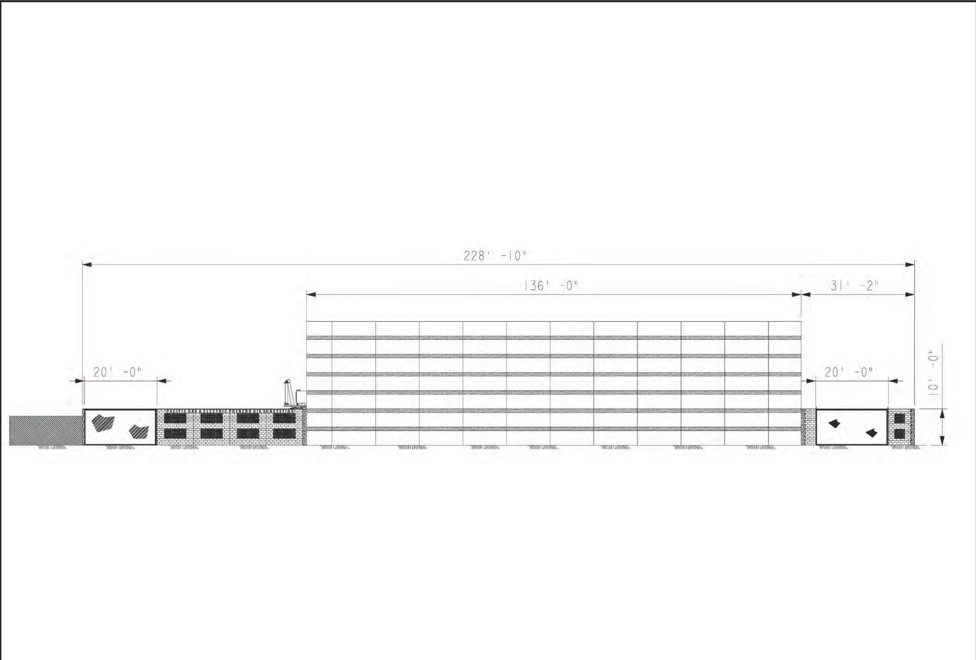
Figure 4-15c Revised Potrero 230 kV Switchyard North Elevation
