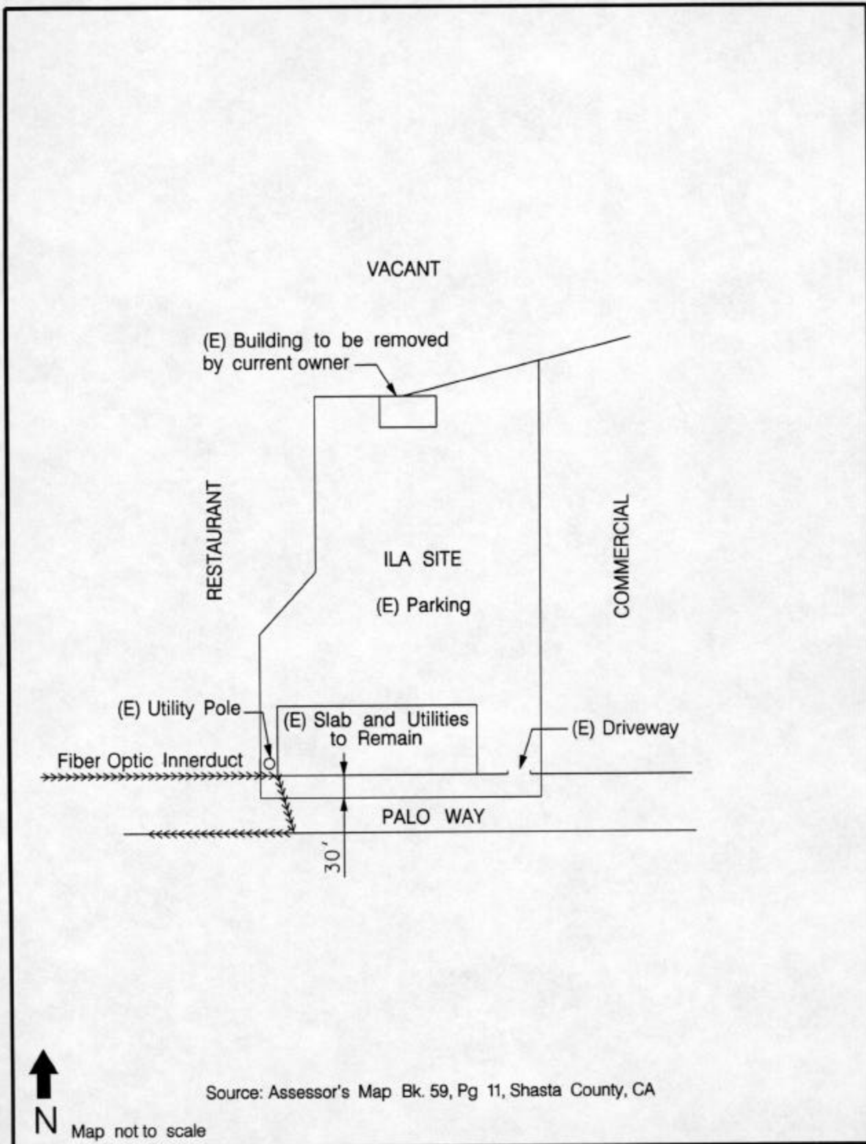
Figure 7: Palo Cedro ILA Conceptual Plot Plan
