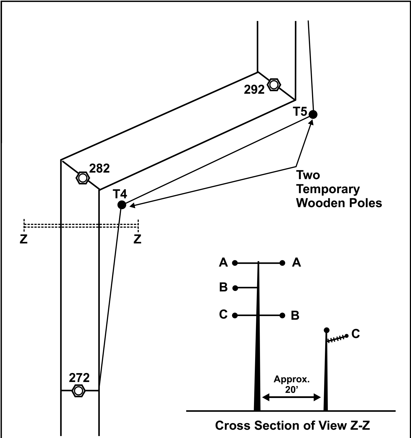
Miguel-Mission 230 kV #2 Project Figure C-1 Pole Placement in the Vicinity of Steele Canyon High School Aspen Environmental Group
