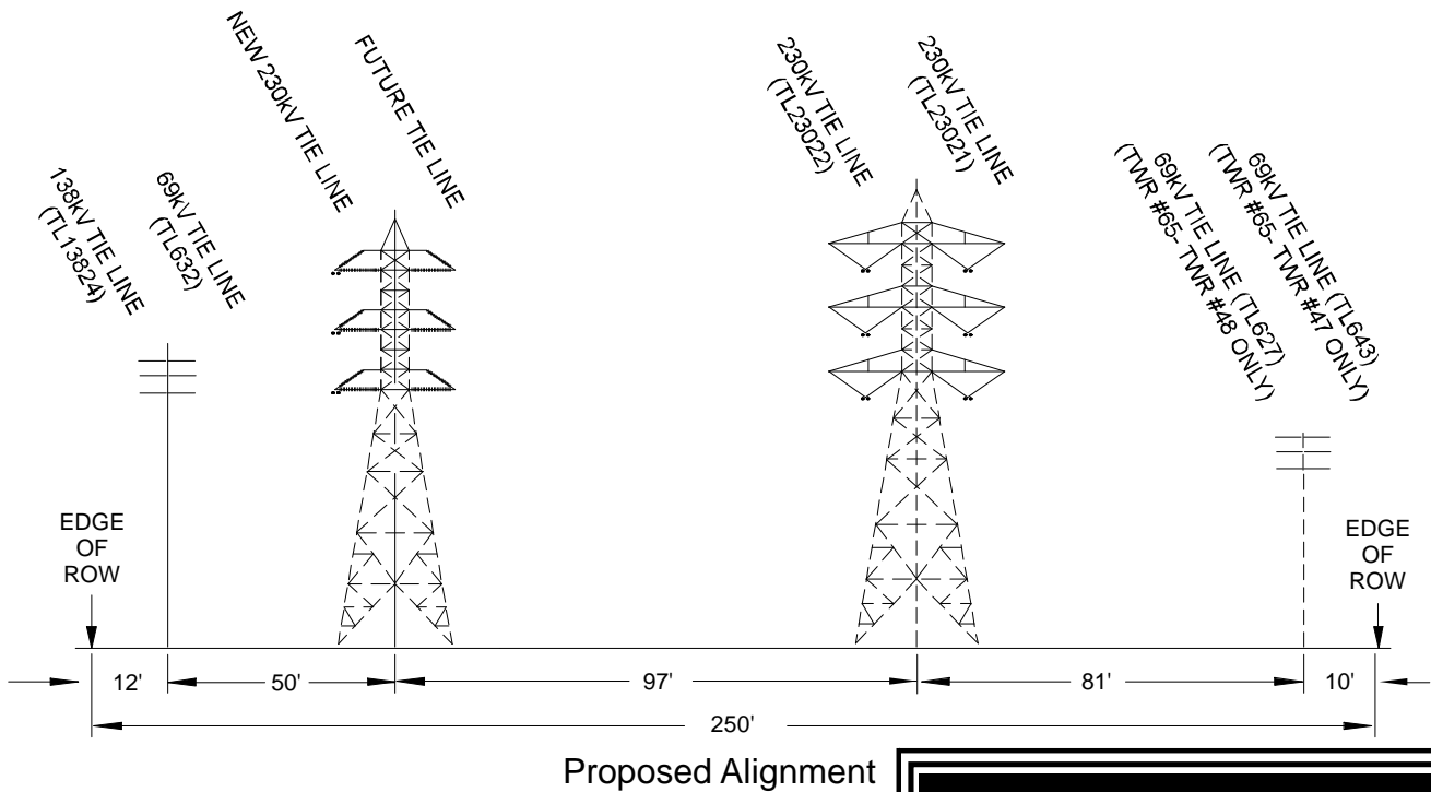
Figure B-8a Existing and Proposed Cross-section of Subsection A (Twr #65 - Twr#49)
