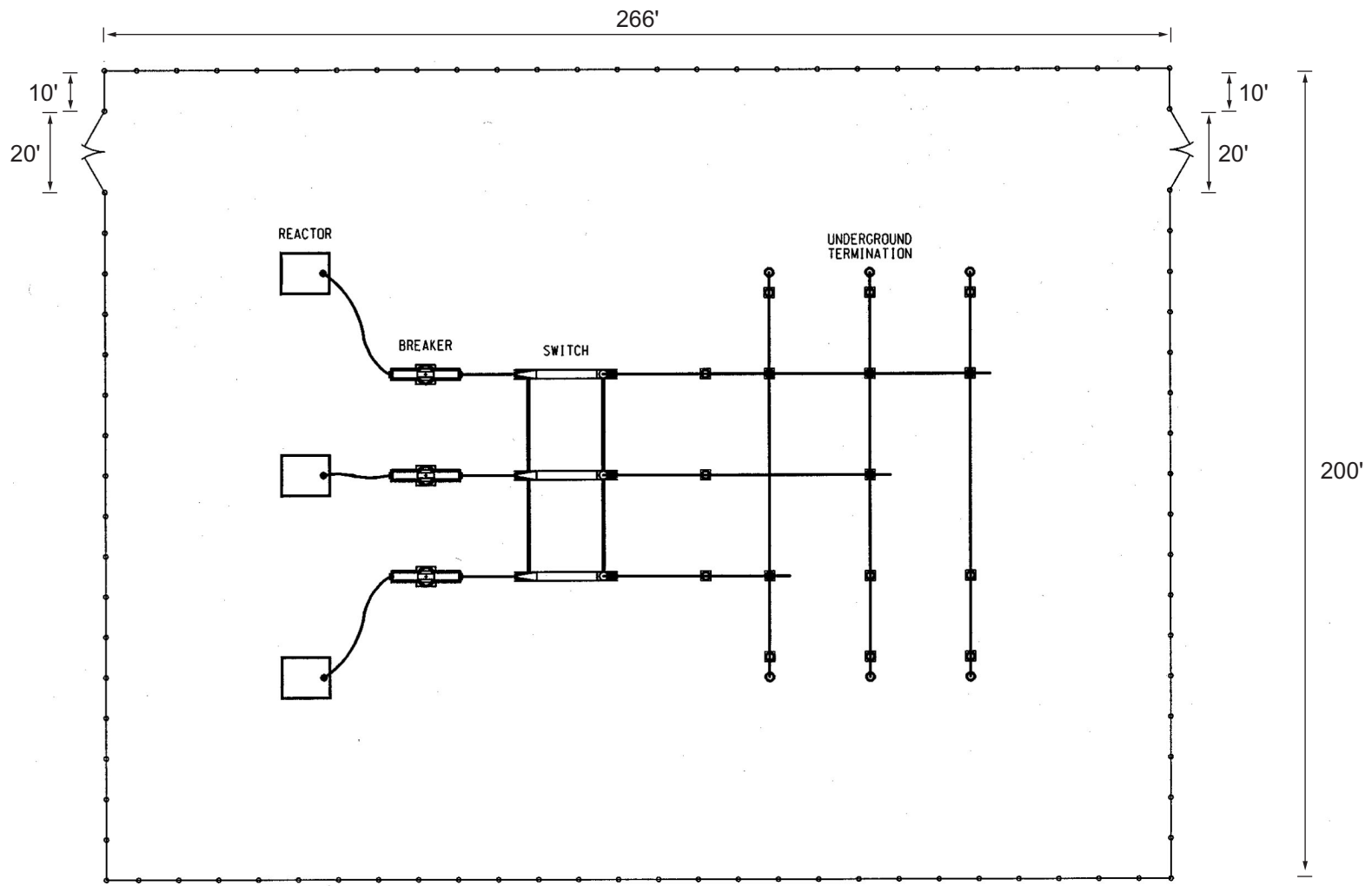
San Diego Gas and Electric Miguel-Mission 230kV #2 Project Figure 3-2: Typical Reactor Station
