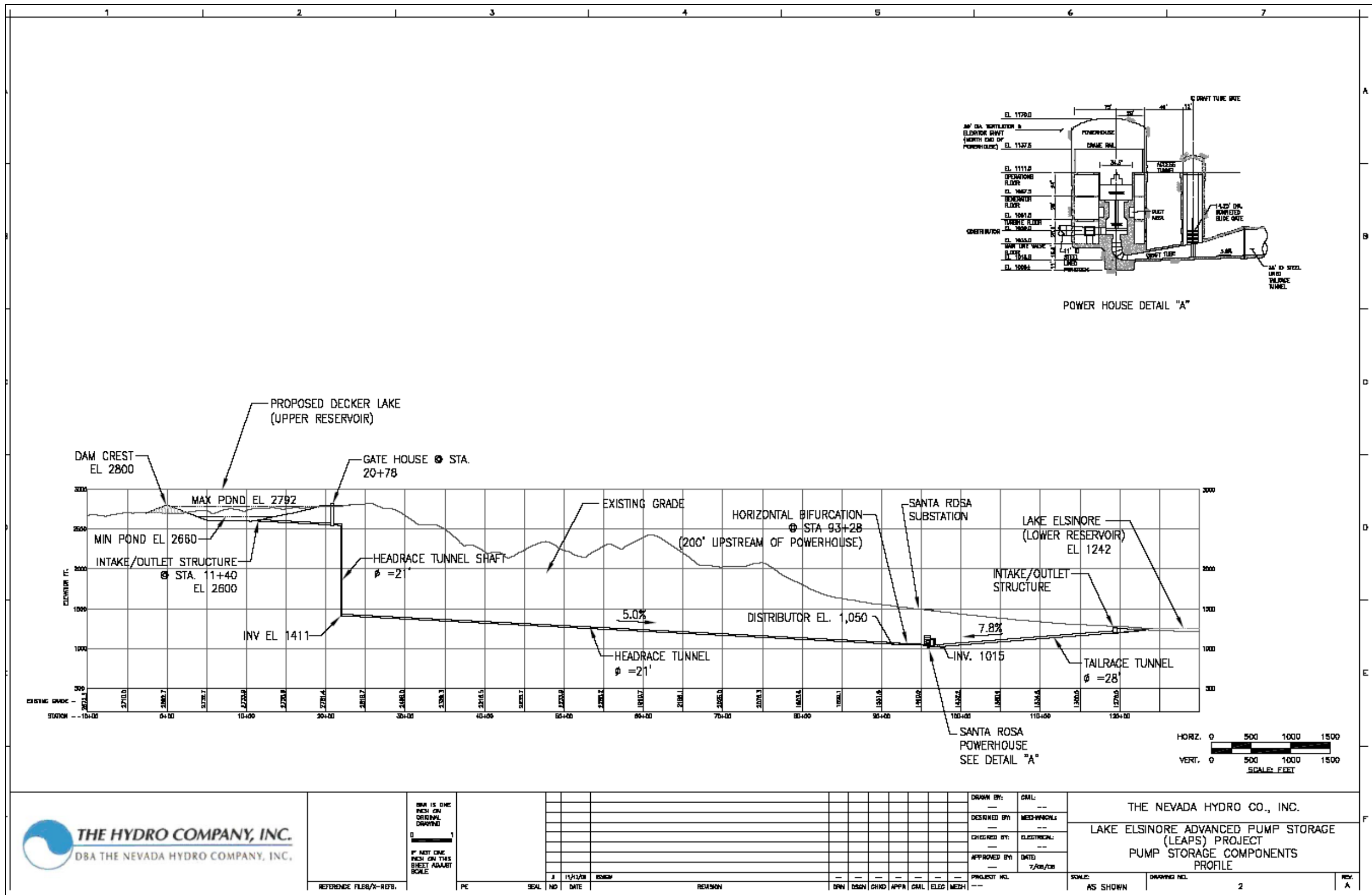
Figure 3.1.1-6: LEAPS Pumped Storage Component (2 of 2)
