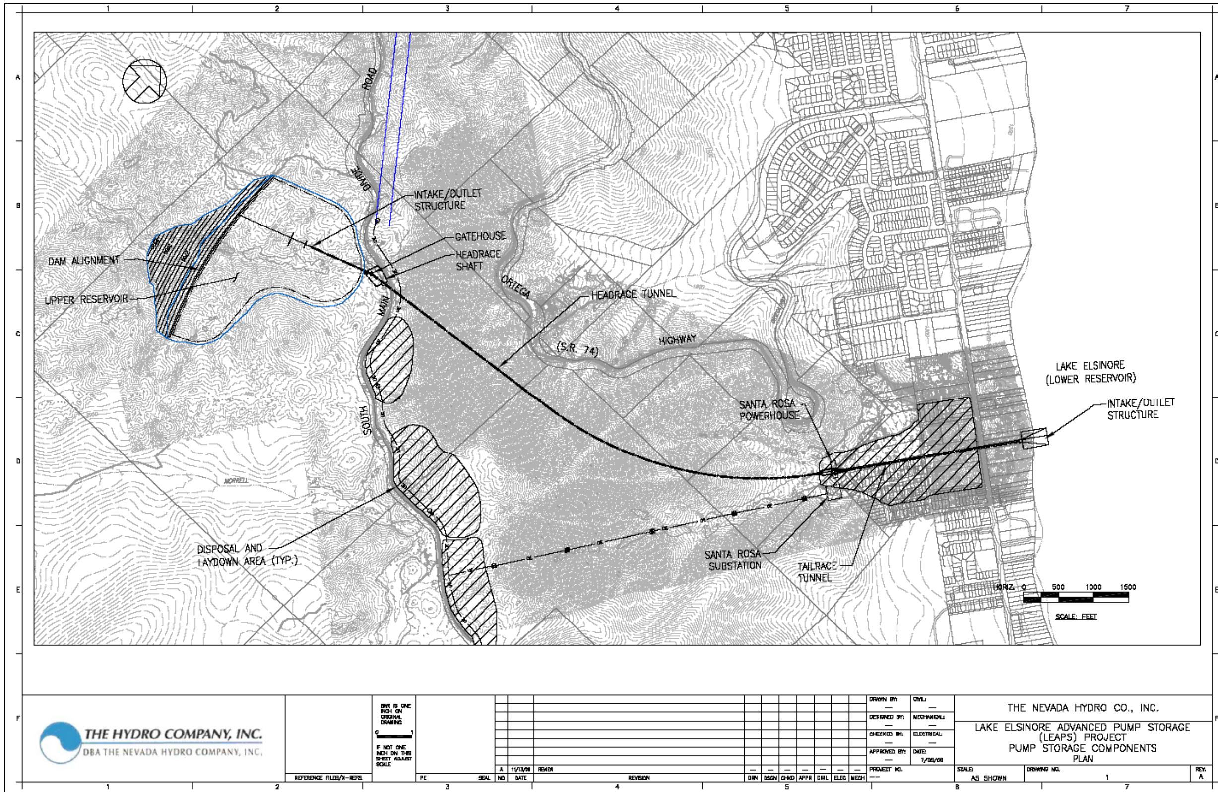
Figure 3.1.1-6: LEAPS Pumped Storage Component (1 of 2)
