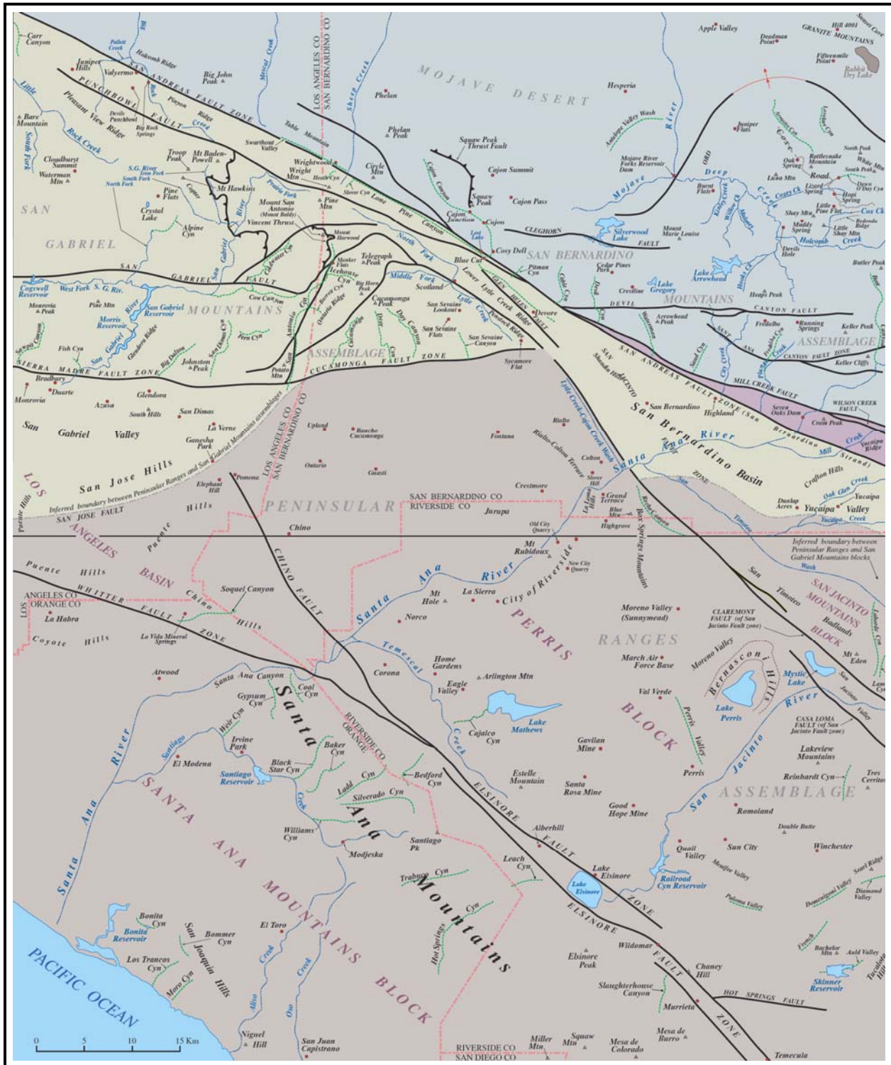
Figure 4.8.1-1. Physiographic Provinces of Southern California Source: United States Geological Survey
