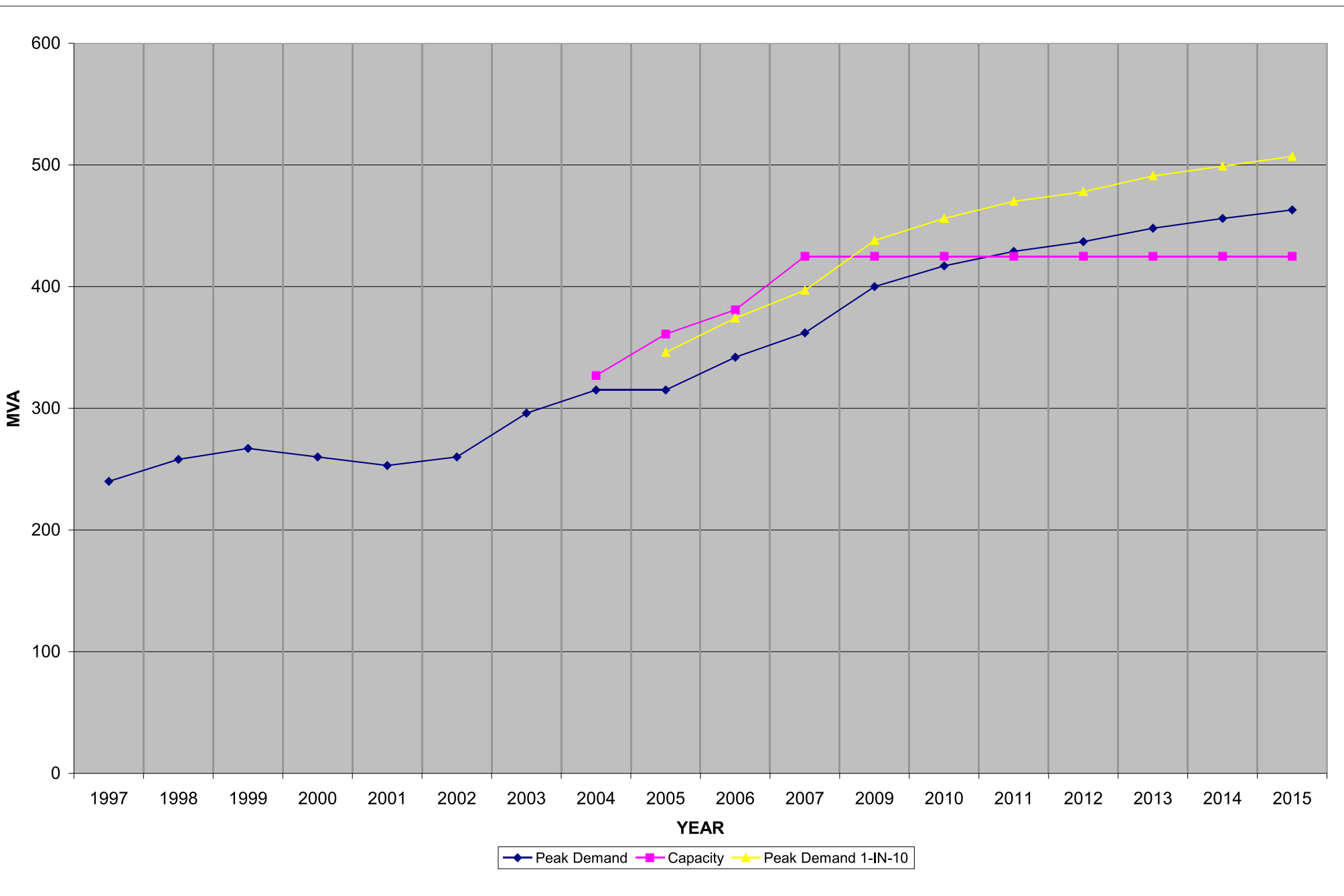
Figure 1-3 Substation Capacity and Peak Demand in Electrical Needs Area
