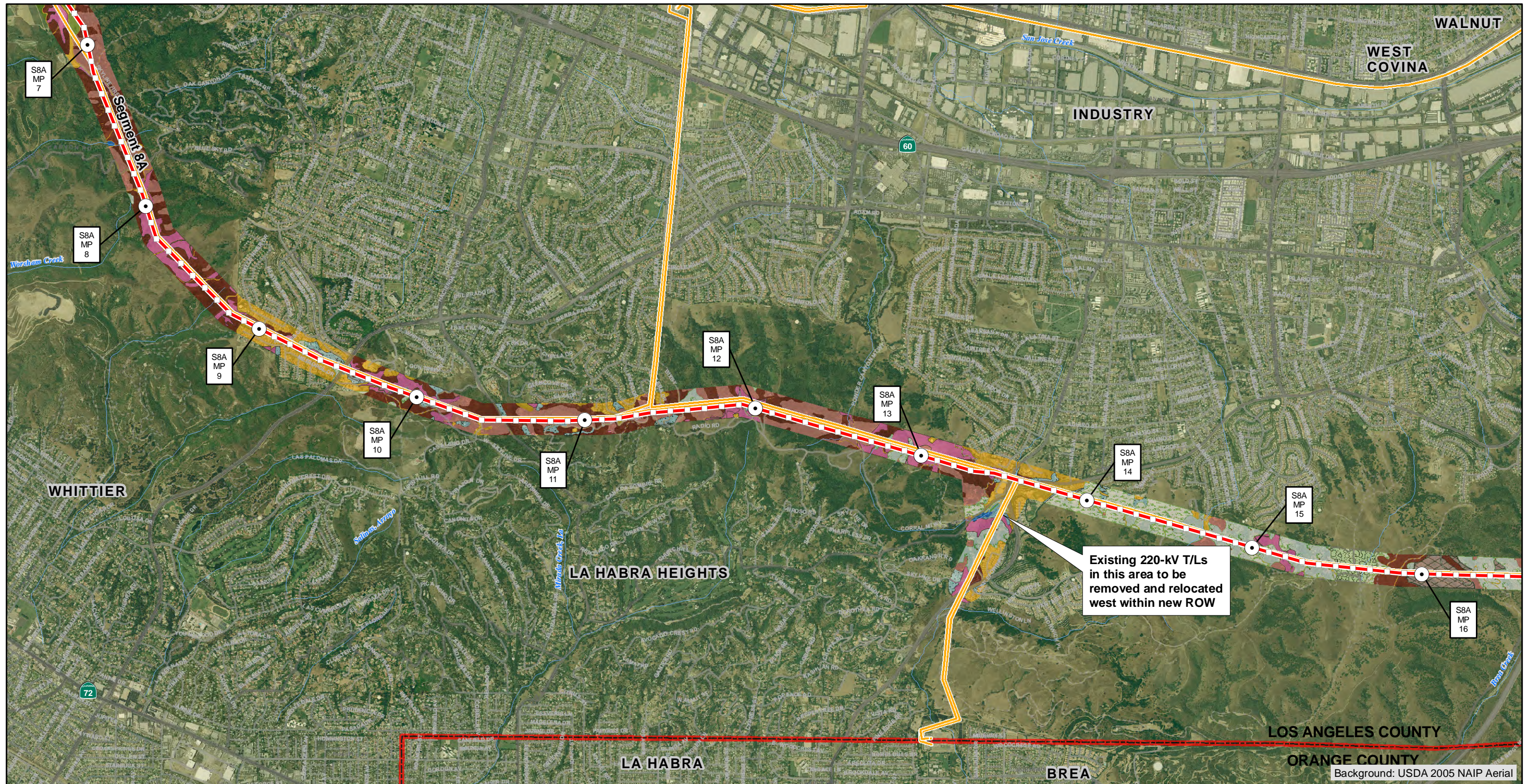
Figure 3.4-4v (Revised) Vegetation Communities Southern Region
