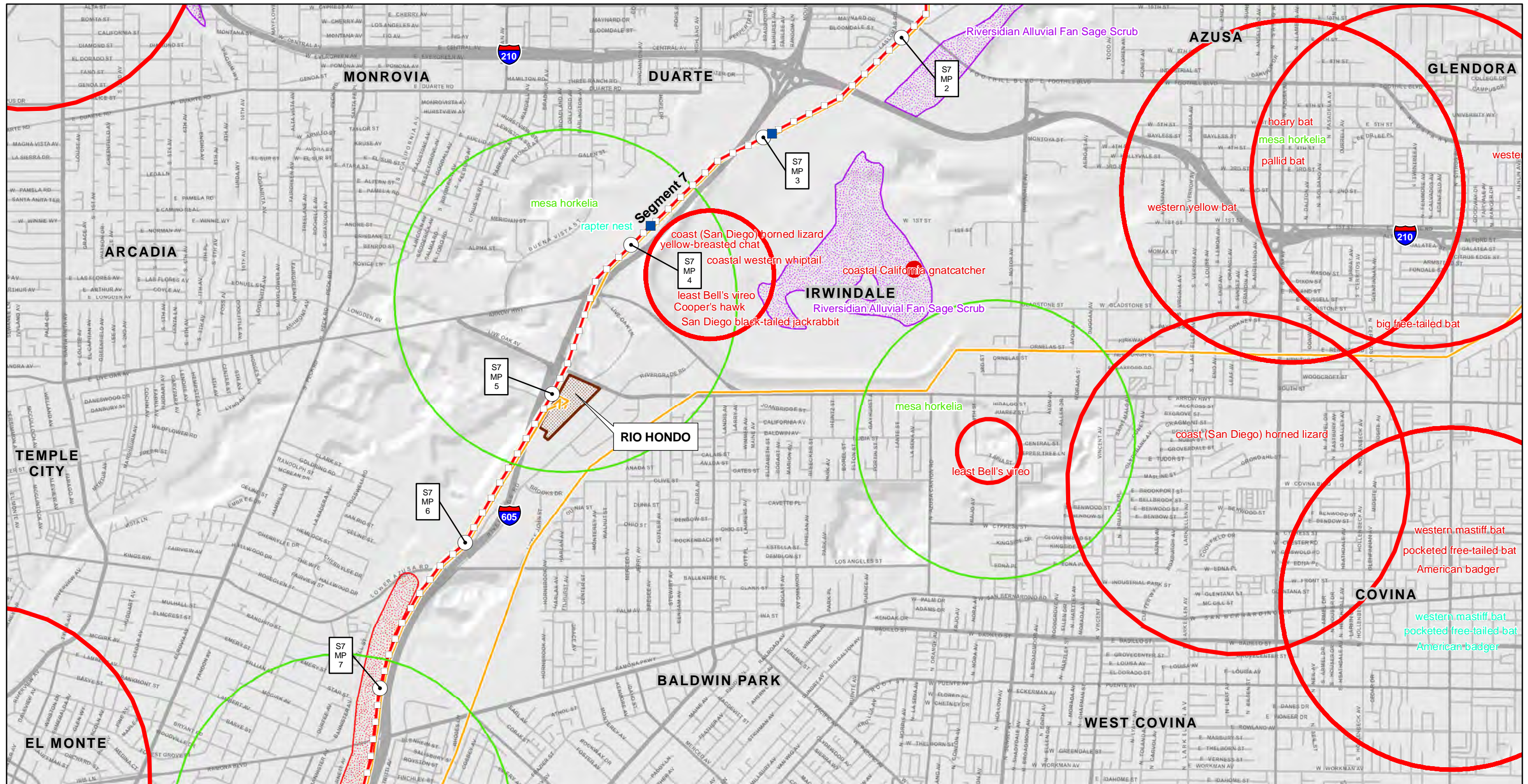
Figure 3.4-5u (Revised) Sensitive Species Locations Southern Region
