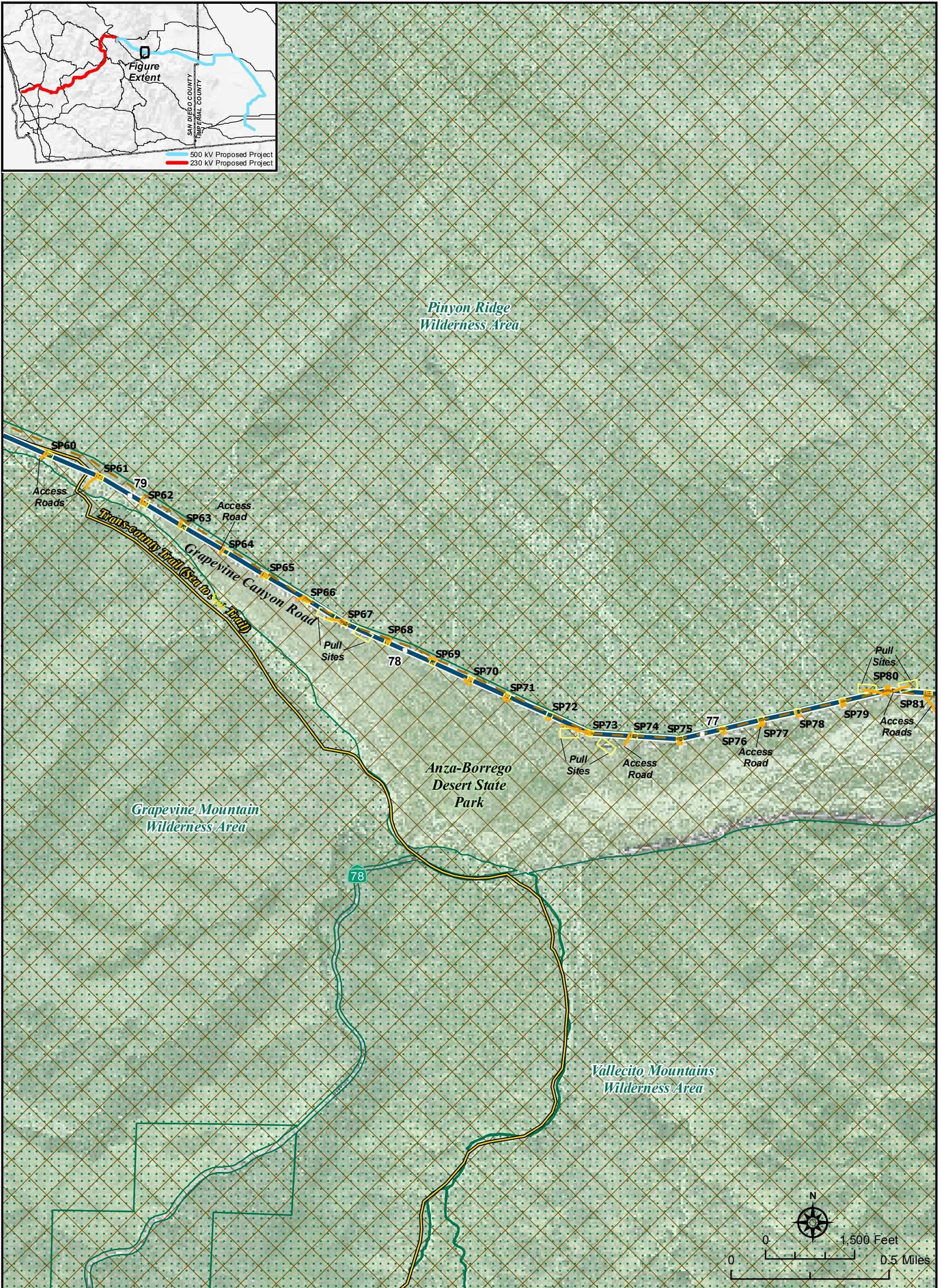
Sunrise Powerlink Project Figure Ap. 11A-20 Proposed Project Detail
