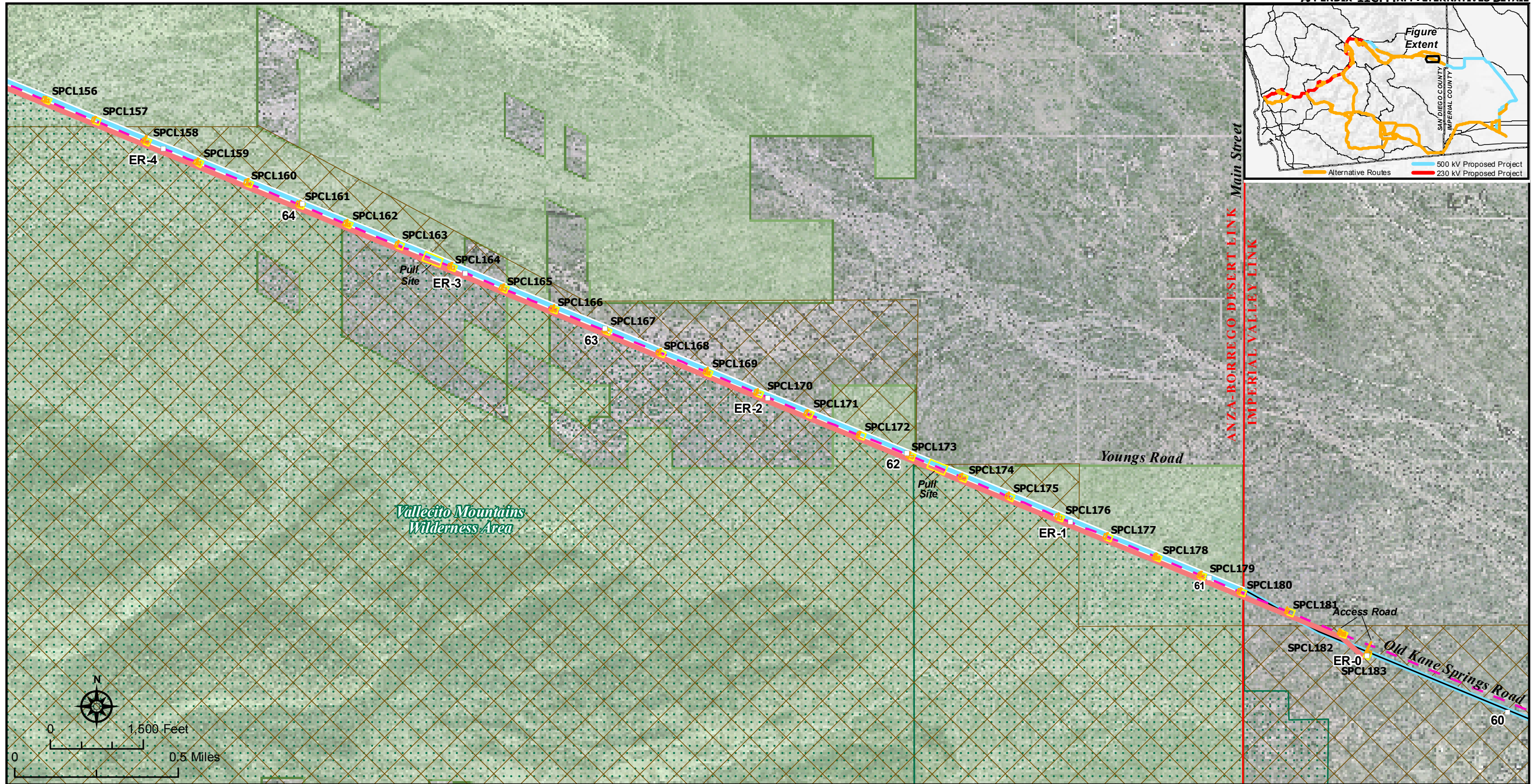
Sunrise Powerlink Project Figure Ap. 11C-14 Overhead 500 kV ABDSP Within Existing ROW Alternative Detail
