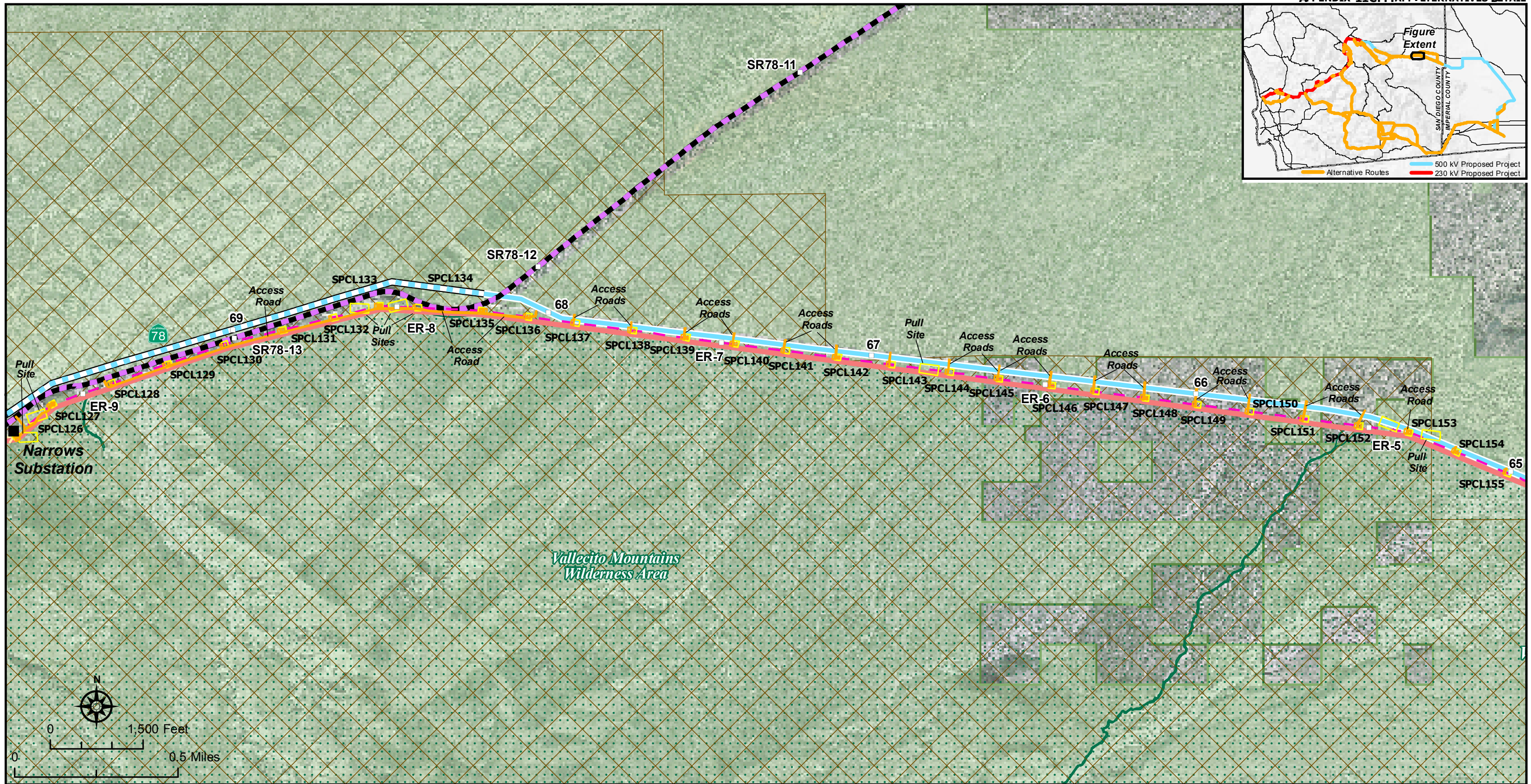
Sunrise Powerlink Project Figure Ap. 11C-15 Overhead 500 kV ABDSP Within Existing ROW Alternative Detail
