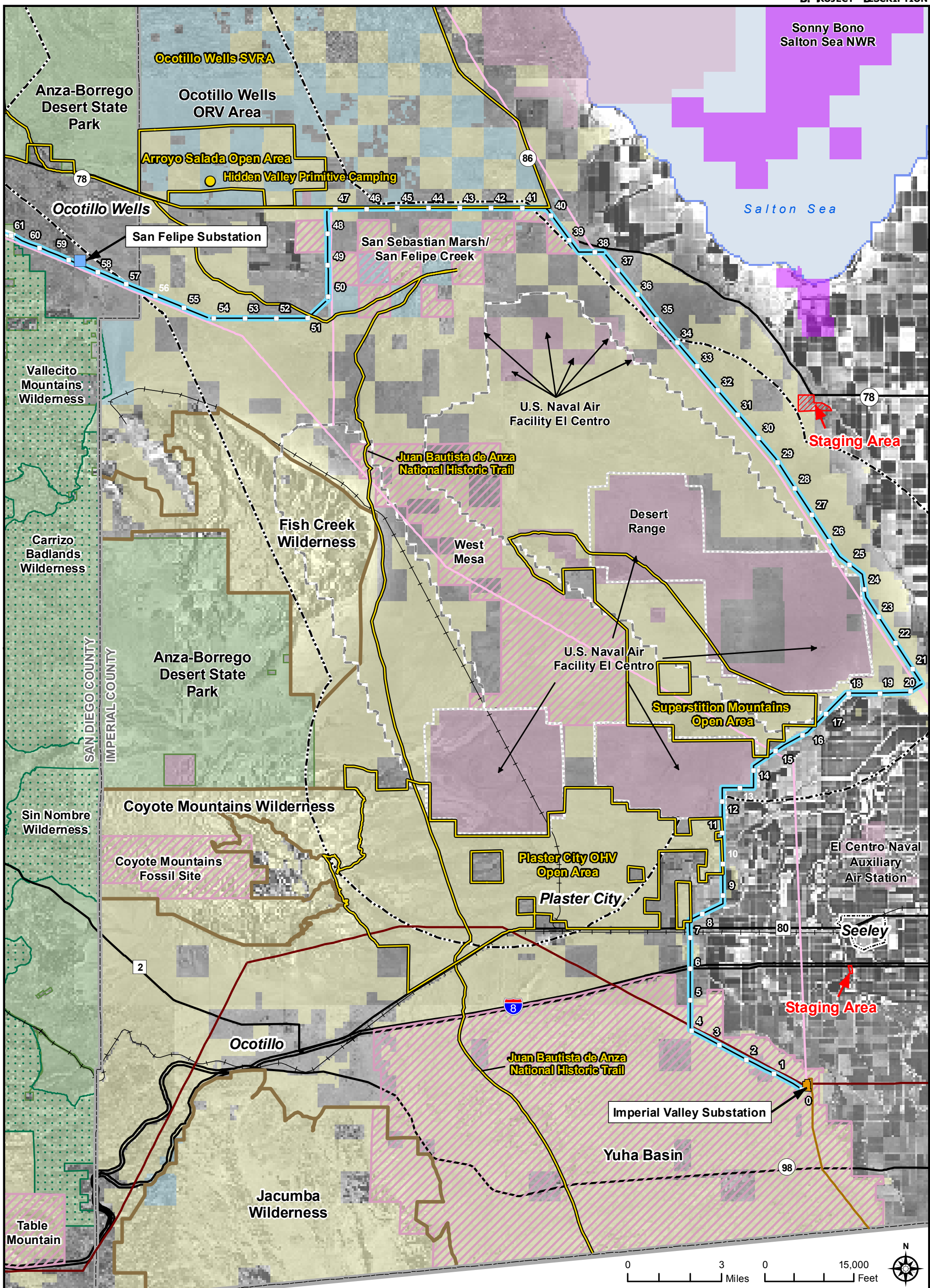
Sunrise Powerlink Project Figure B-3 Imperial Valley Link
