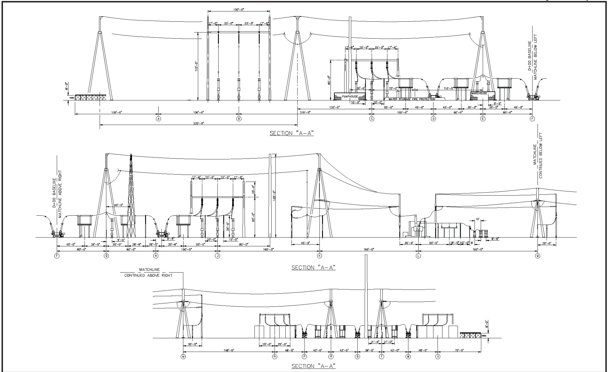
Sunrise Powerlink Project Figure B-33 Central East Substation: 500/230 kV Switchyard: Section A-A
