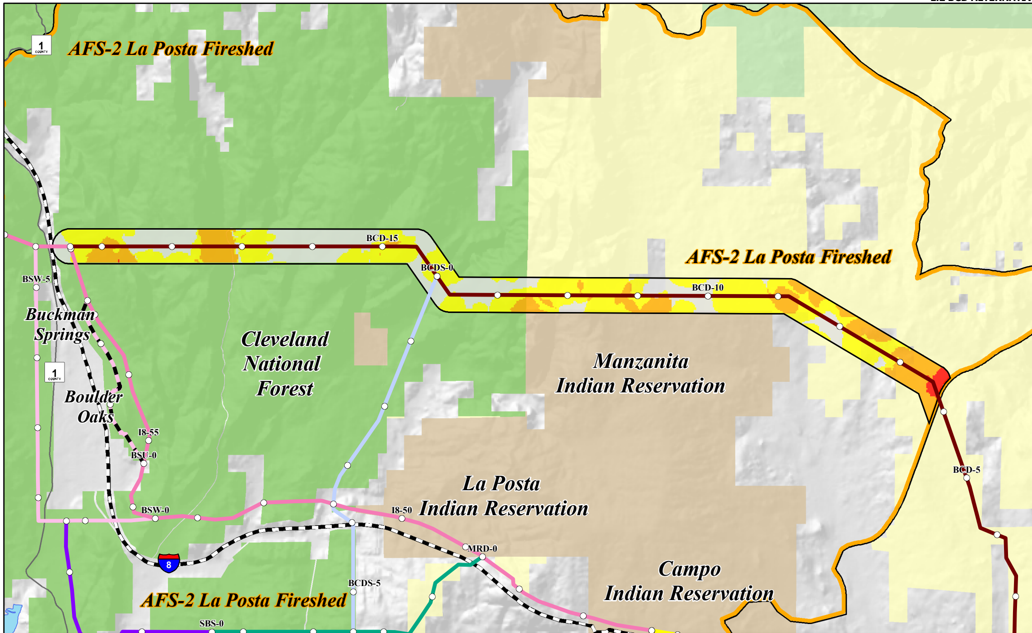
Sunrise Powerlink Project Figure E.2.15-3 La Posta Fireshed BCD Alternative Burn Probability Model
