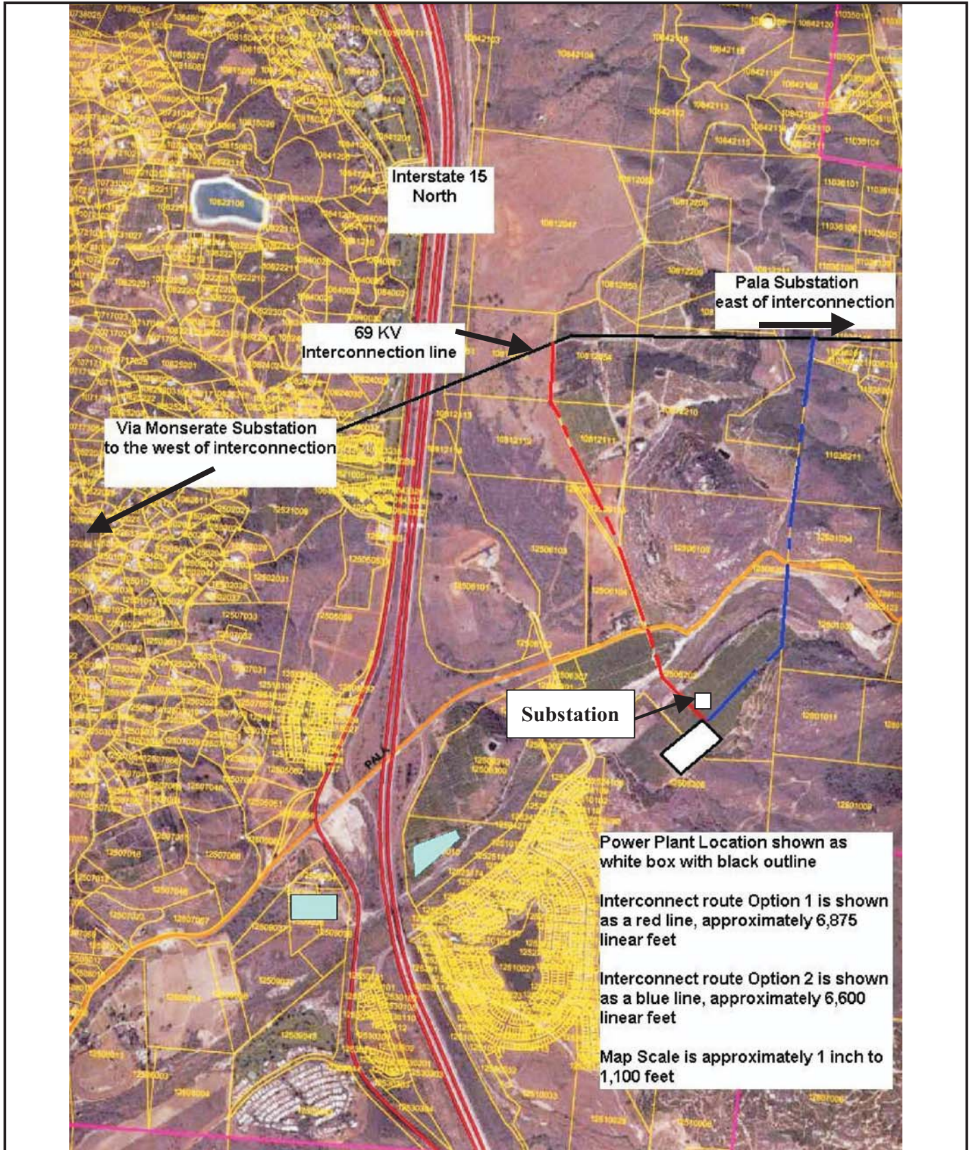
Figure E.5.1-3c Location of Fallbrook Energy Facility Potential Interconnections
