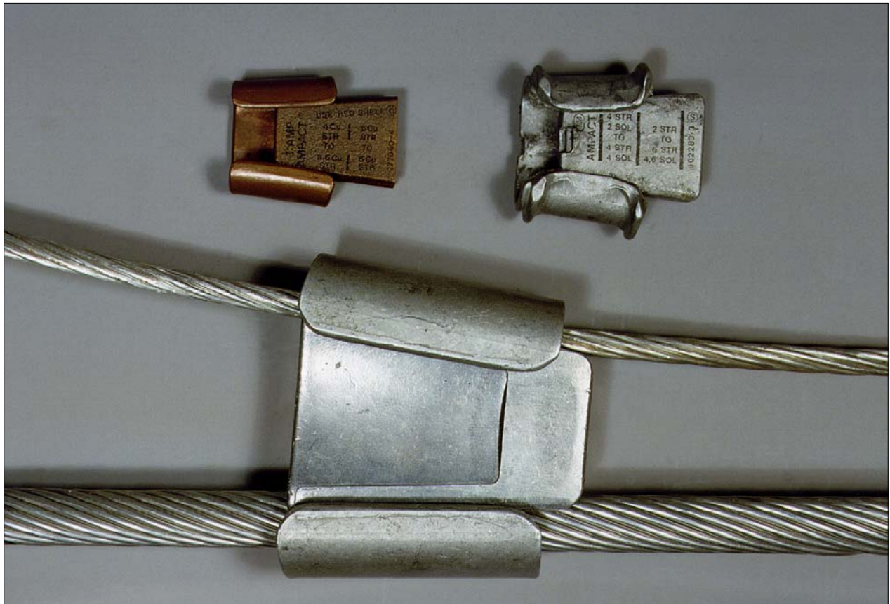
Figure 3-40 Fired Wedge Connectors
