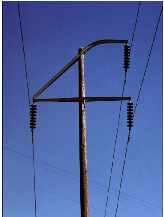
Figure 4-22 Triangular Post
