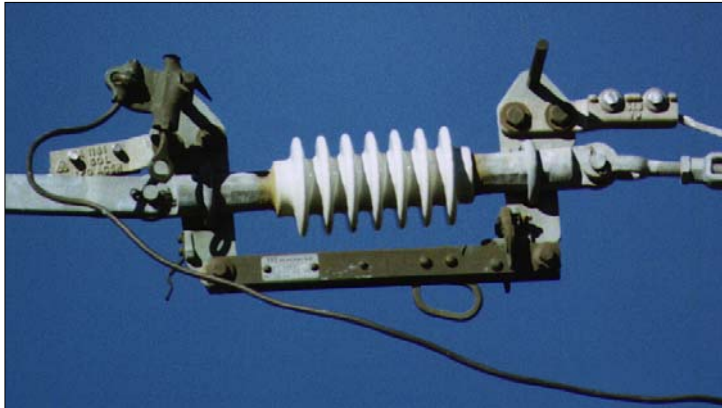
Figure 2-12 In-Line Disconnect (closed position)
