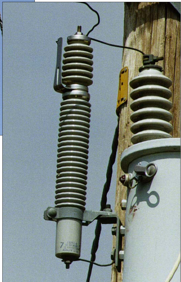
Figure 2-23 Gapped Lightning Arrester
