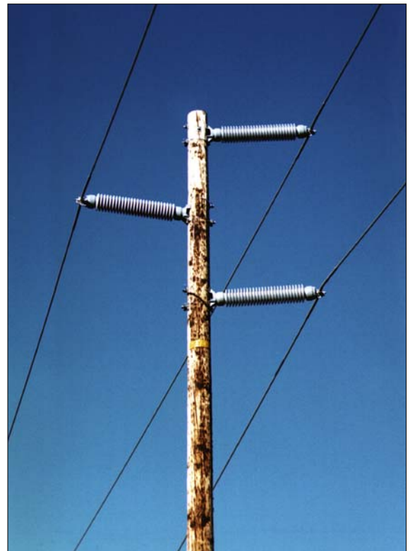
Figure 4-22 Triangular Post
