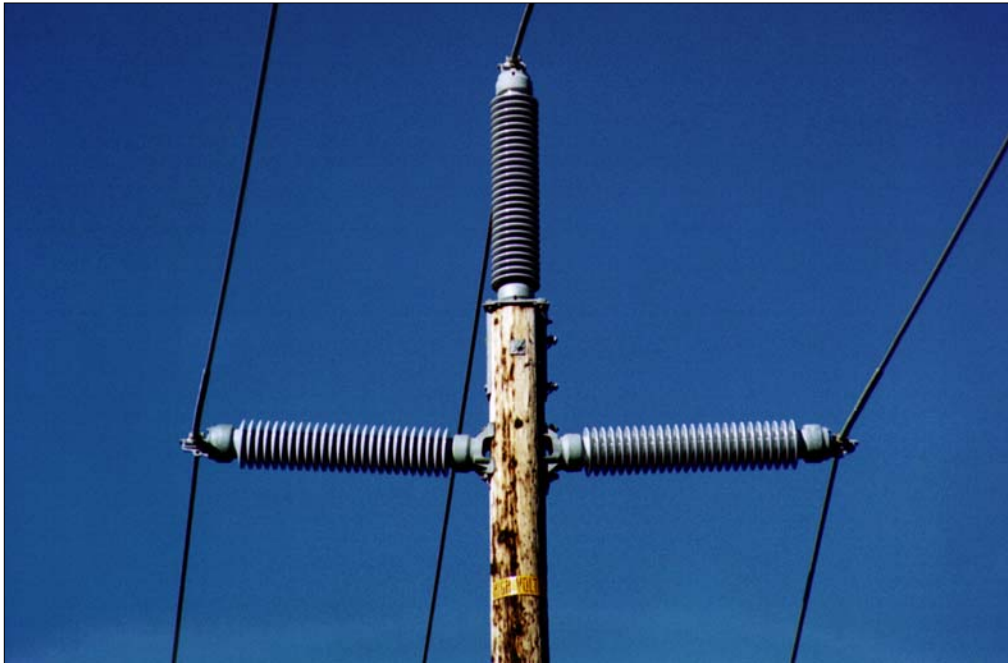
Figure 4-23 Triangular Configuration
