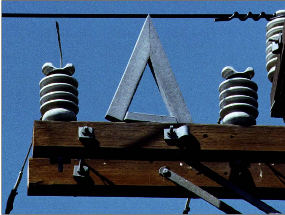
Figure 4-17 Anti-Perch Guard
