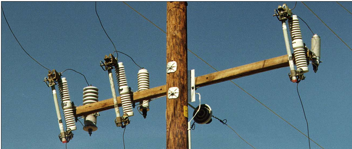
Figure 3-10 Arm Mounted Cutout with SMU-20 Fuses
