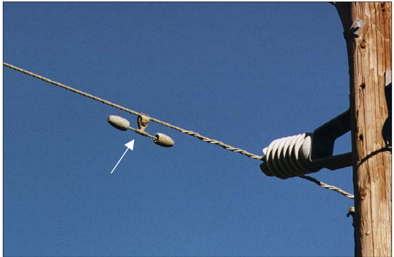
Figure 4-14 Vibration Damper
