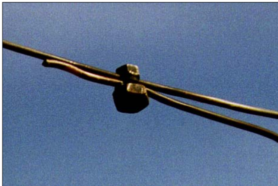
Figure 2-28 Split Bolt Connector
