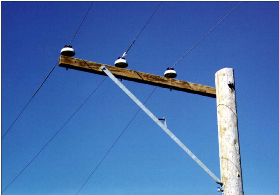
Figure 4-3 Alley Arm
