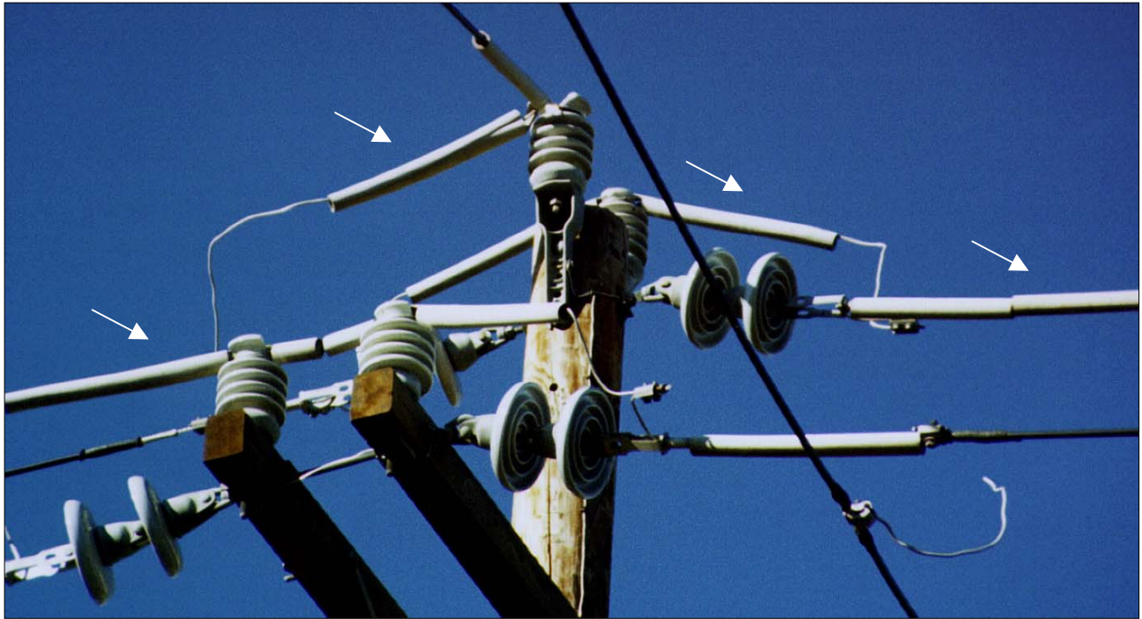
Figure 4-15 Insulated Conductor Covering
