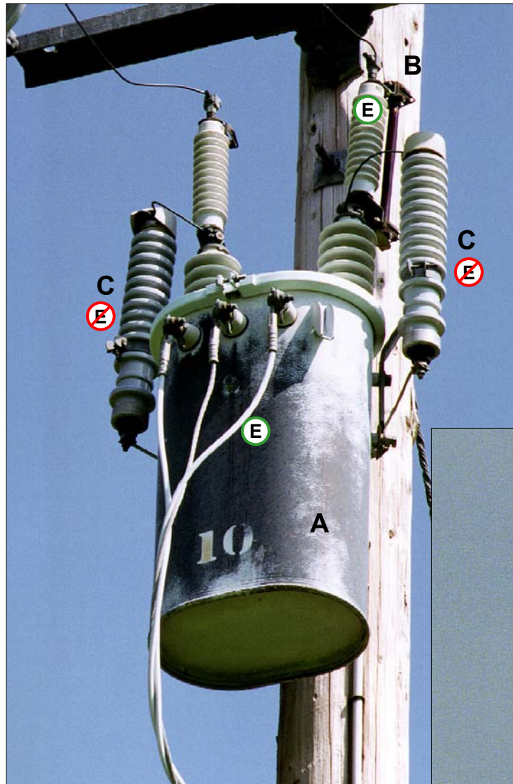
Figure 2-22 Transformer Mounted Lightning Arrester A. Conventional Transformer (E) B. Bushing Mounted Liquid Filled Fuse (E) C. Lightning Arresters (E)
