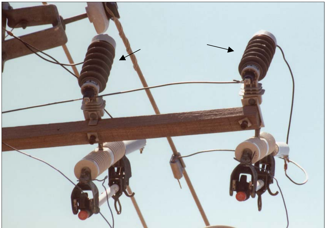
Figure 2-21 Non-Porcelain Lightning Arrester
