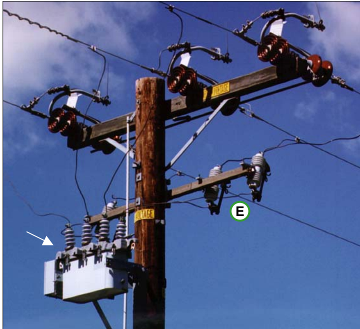
Figure 3-25 Sectionalizer with Solid Blade Disconnects
