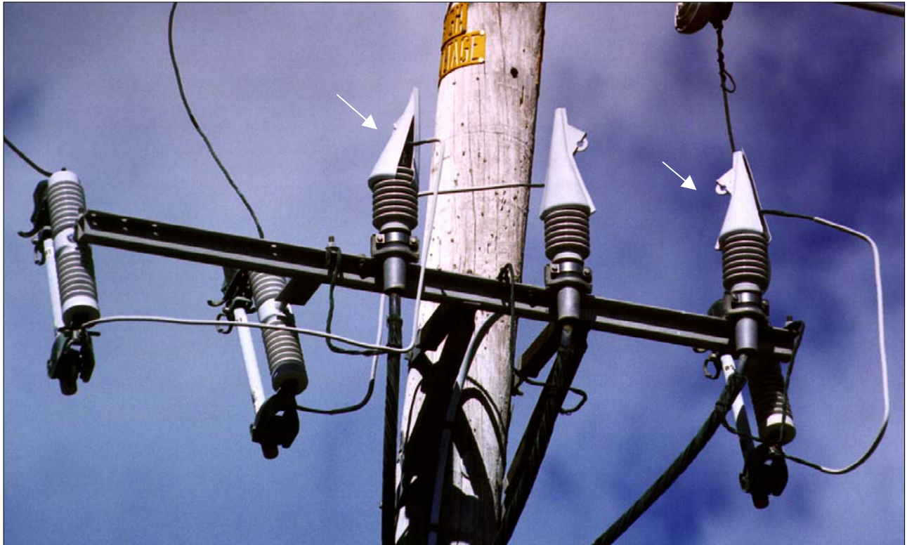
Figure 4-19 Squirrel Guard
