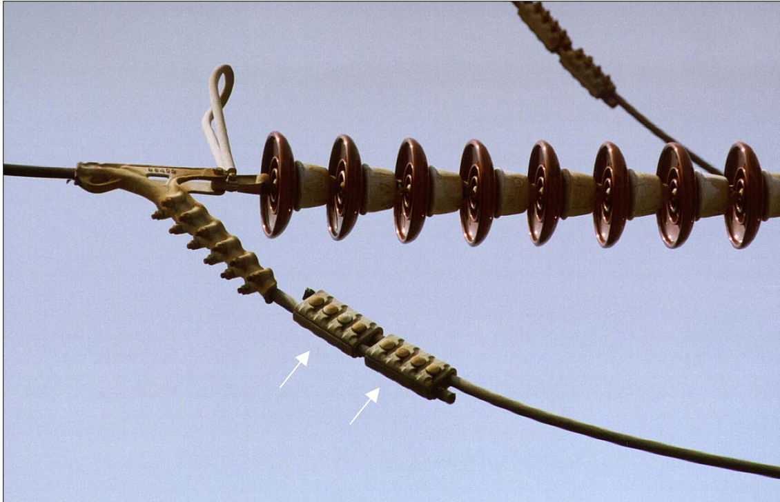
Figure 3-34 Transmission Deadend with Parallel Groove Connectors
