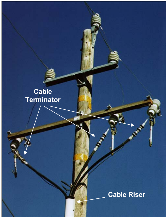
Figure 4-9 Cable Riser with Cable Terminator
