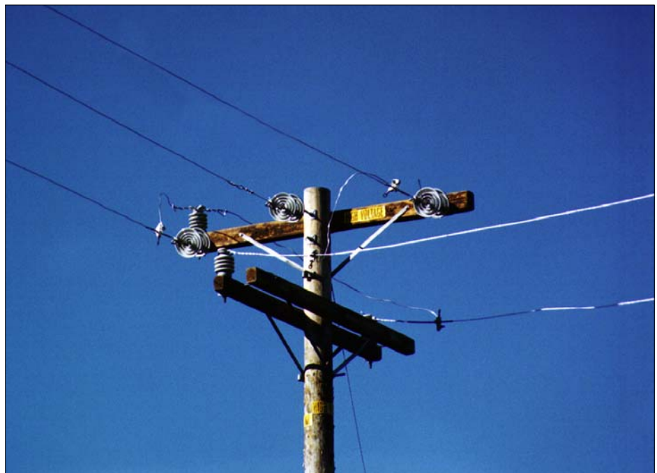
Figure 4-6 Crossarm Deadend Corner (Line and Buck)
