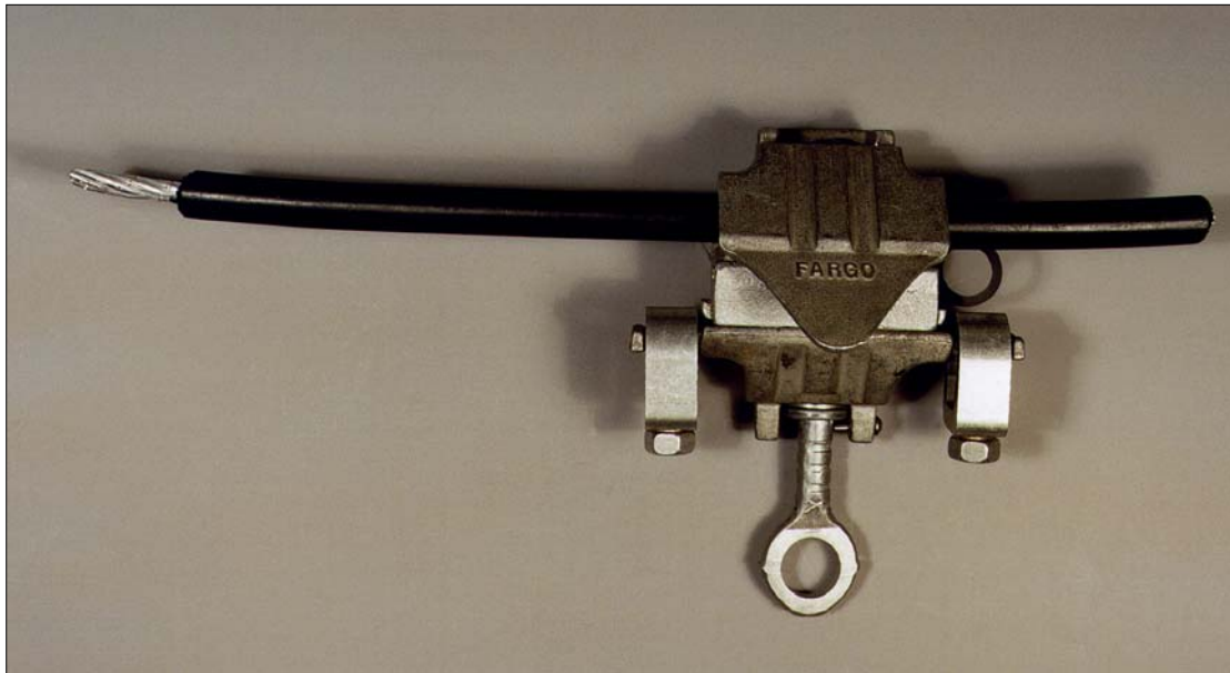
Figure 3-36 Piercing Hot Tap Clamp on Tree Wire
