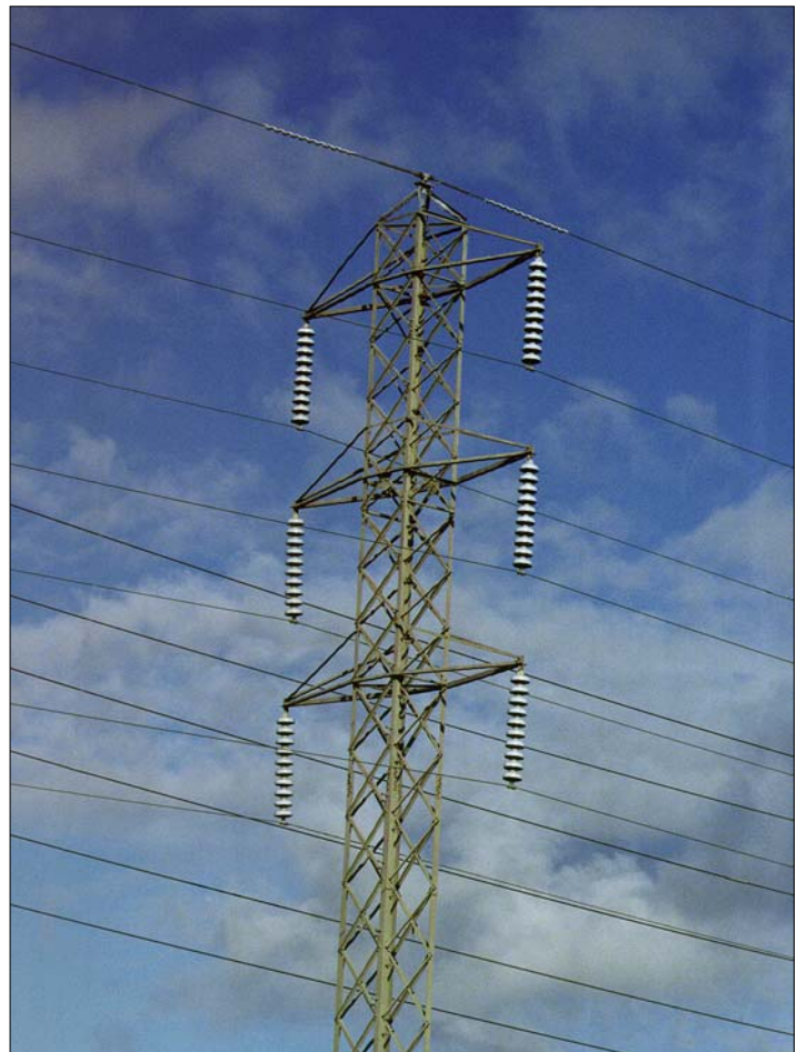
Figure 4-27 Tangent Transmission Tower with Static Line
