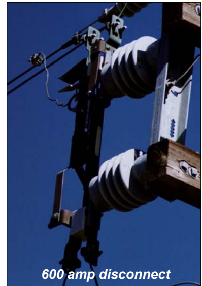
Figure 2-10 Solid Blade Disconnects
