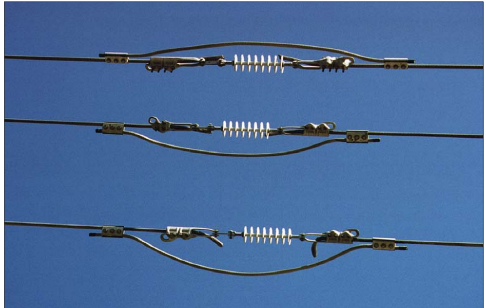
Figure 4-11 Line Opener
