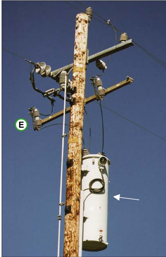
Figure 3-27 Voltage Regulator with Solid Blade Disconnects
