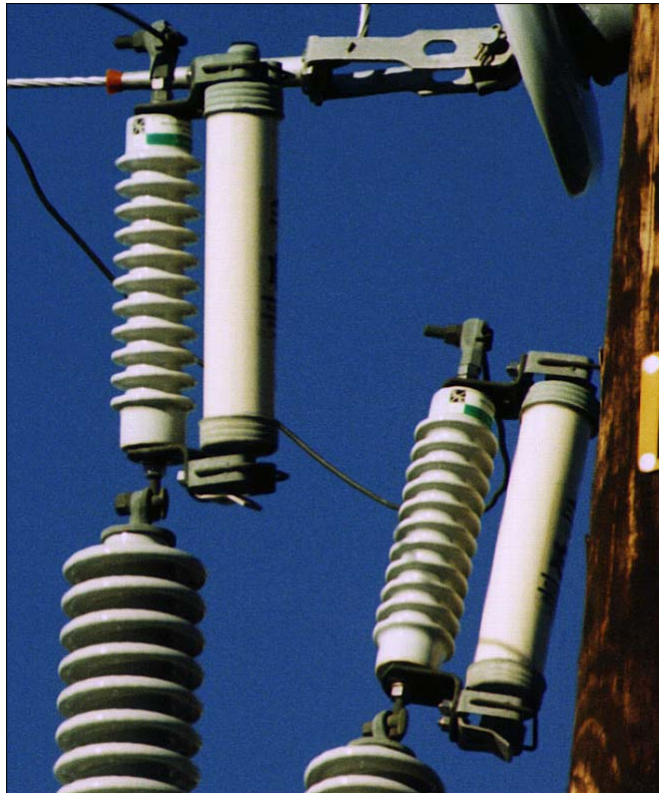
Figure 3.4 Bushing Mounted Cutout with Non-Expulsion Fuse
