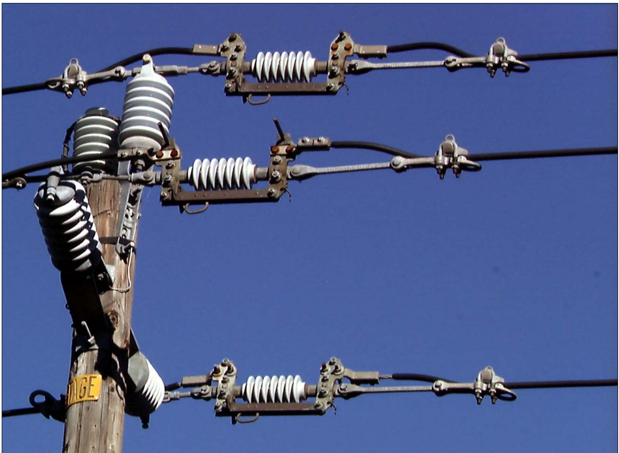
Figure 2-13 In-Line Disconnects (closed position)
