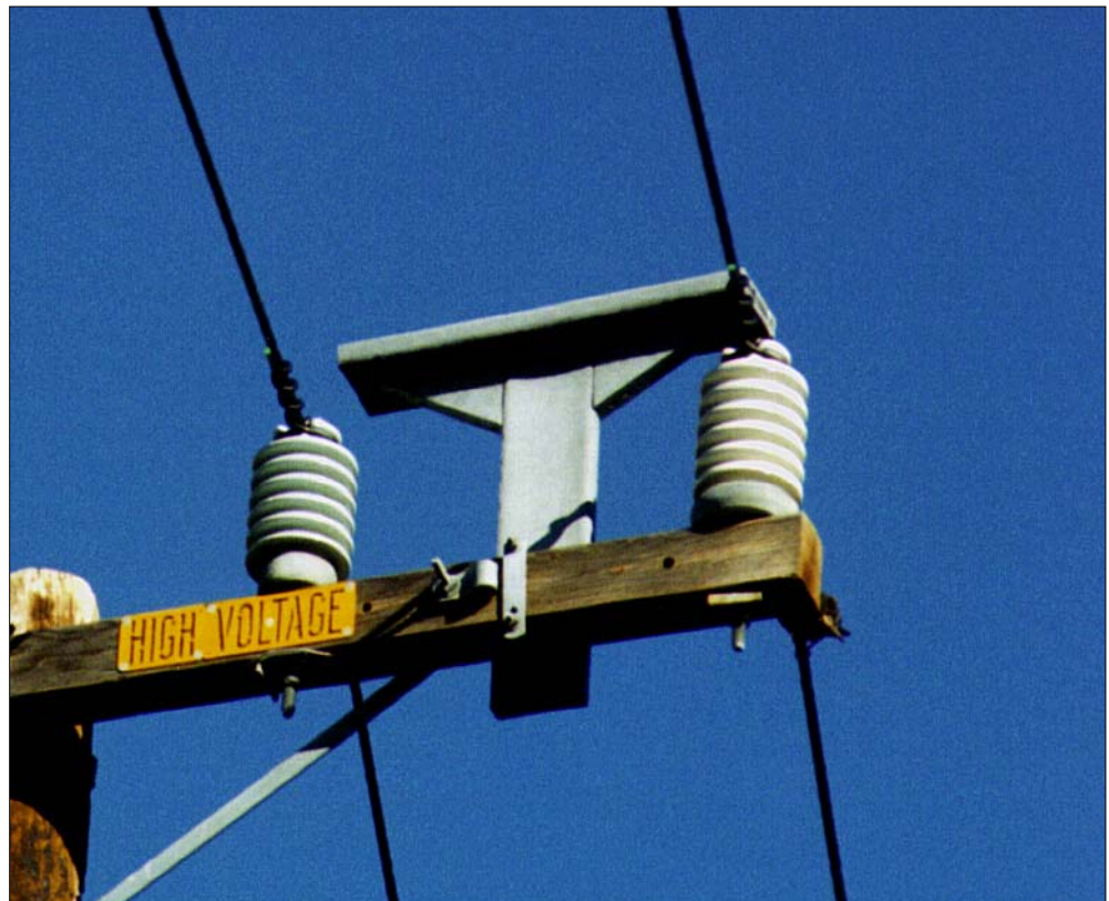
Figure 4-16 Raptor Perch
