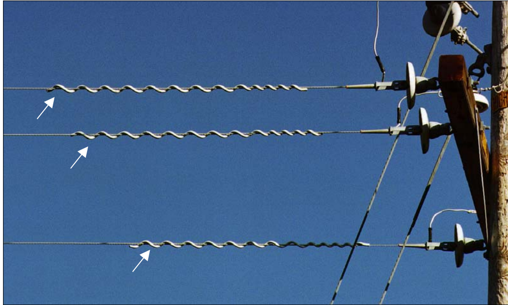
Figure 4-13 Vibration Damper
