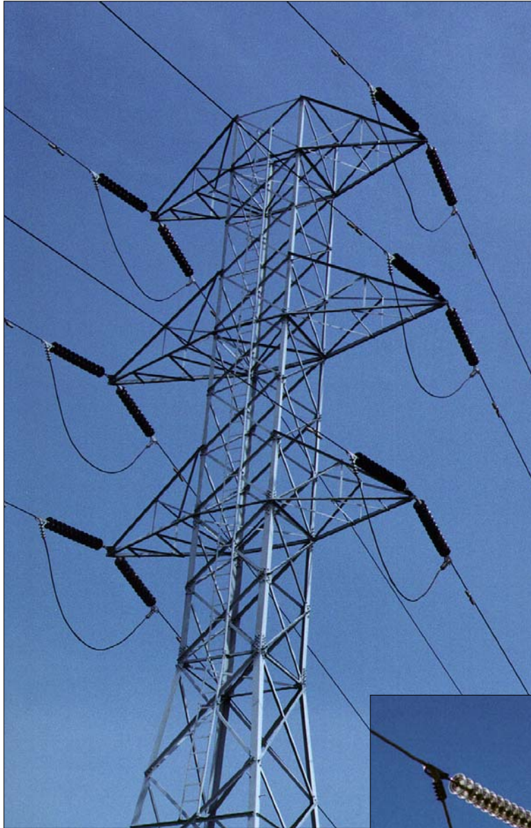
Figure 4-26 Deadend Tower
