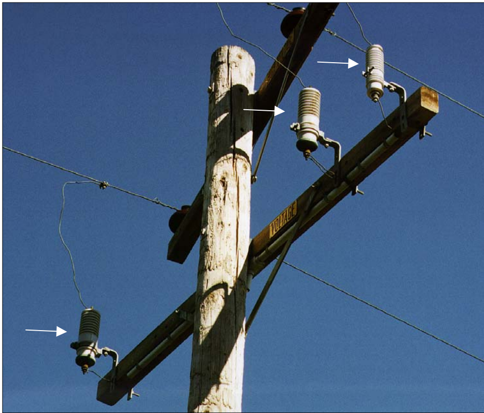
Figure 2-18 Lightning Arrester
