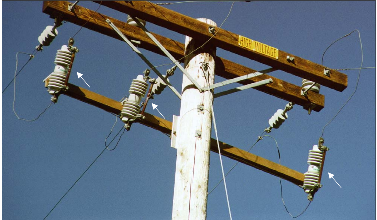
Figure 3-6 Arm Mounted Cutout with Liquid Filled Fuse
