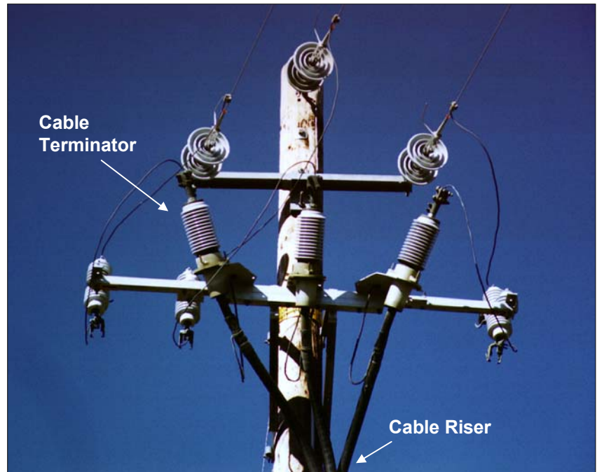
Figure 4-10 Cable Riser with Cable Terminator
