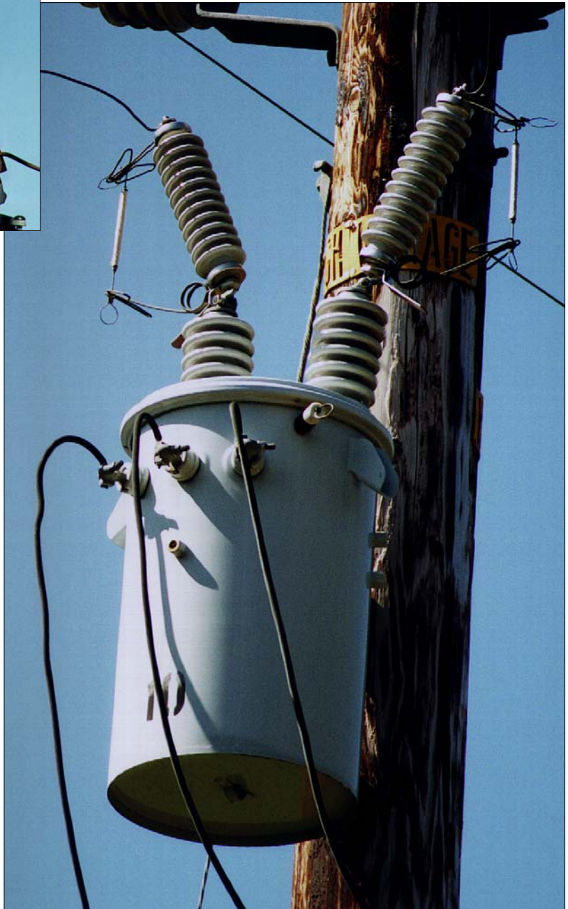
Figure 2-5 Bushing Mounted Cutout with Open Link Fuses
