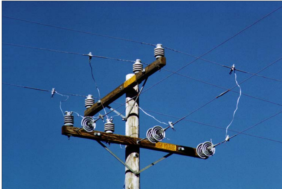
Figure 4-5 Tangent Crossarm with Deadend Tap (T-Tap)
