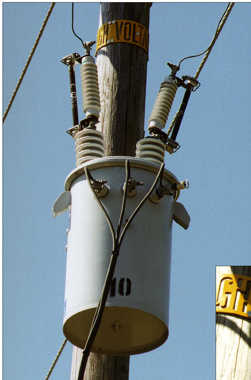
Figure 3-7 Bushing Mounted Cutout with Liquid Filled Fuse
