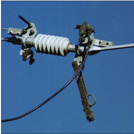
Figure 2-14 In-Line Disconnect (open position)
