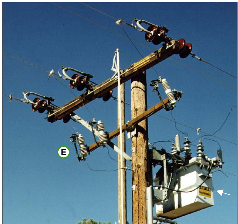
Figure 3-24 Recloser with Solid Blade Disconnects (closed position)
