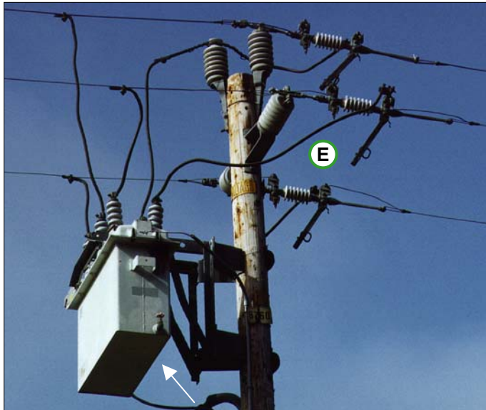
Figure 3-24 Recloser with Solid Blade Disconnects (closed position)
