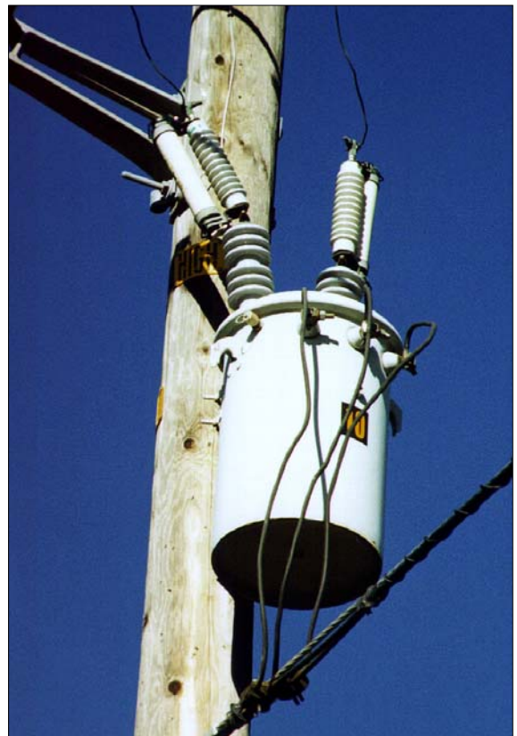
Figure 3-5 Bushing Mounted Cutout with Non-Expulsion Fuses
