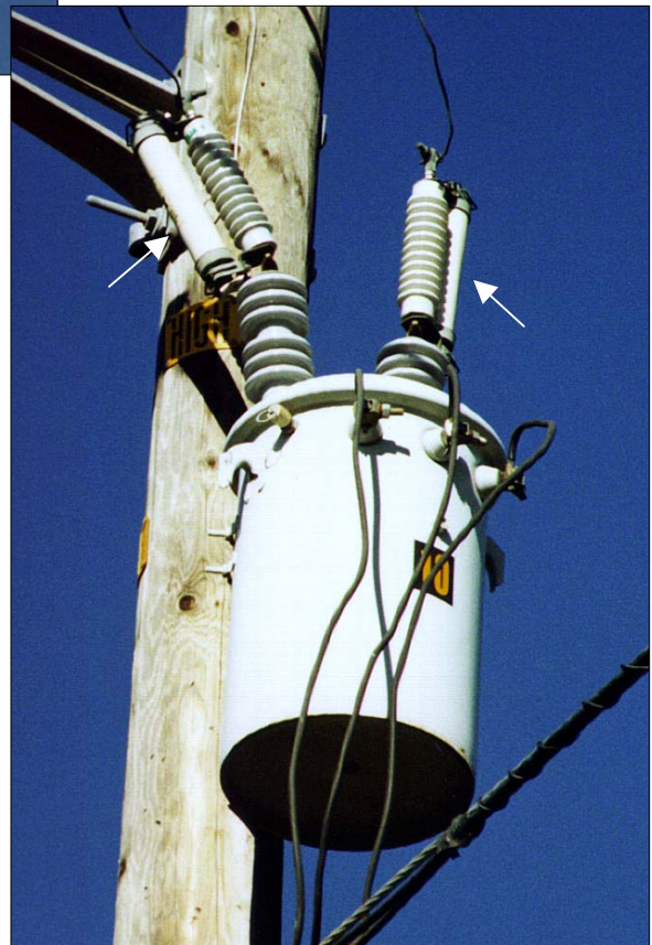
Figure 3-31 Conventional Transformer with Exempt Fuses
