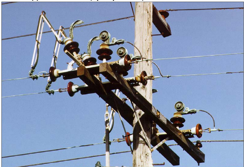
Figure 2-32 Grasshopper Air Switch (open position)
