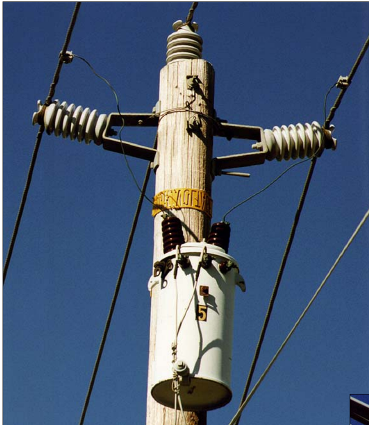
Figure 3-30 Self-Protected Transformer (no external cutouts or fuses)
