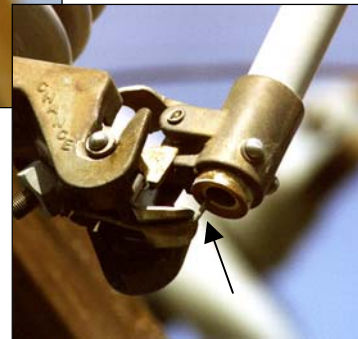
Figure 2-2 Universal Fuse, Fuse link, Expulsion end of fuse
