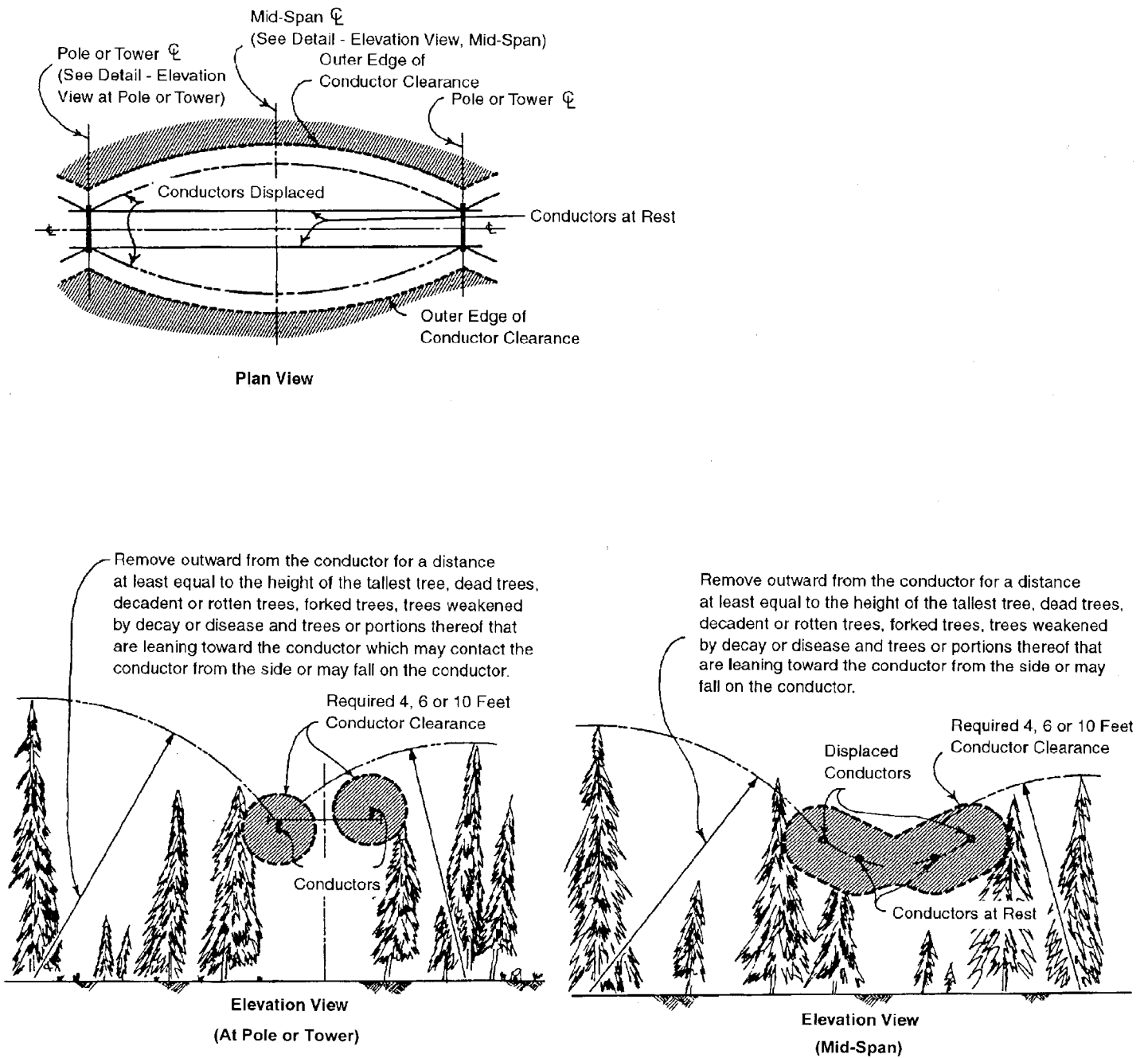
Figure 9 PRC 4293 14 CCR 1256 Conductor Clearance
