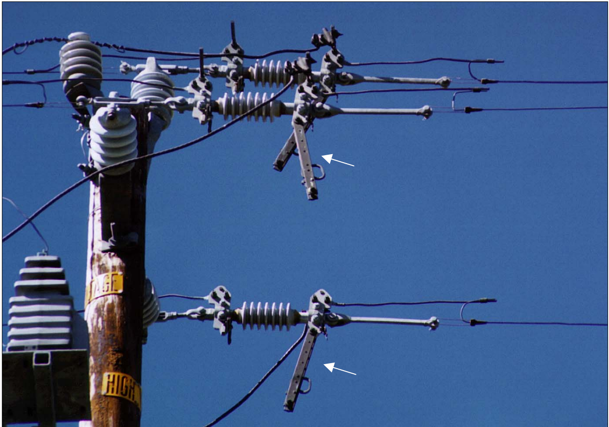
Figure 2-15 In-Line Disconnects (open position)
