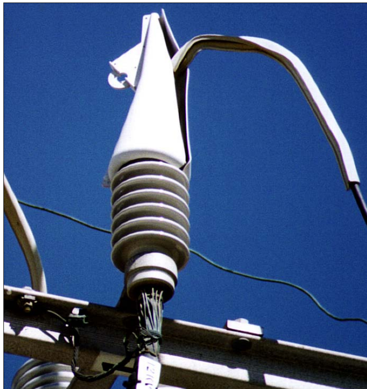
Figure 4-19 Squirrel Guard
