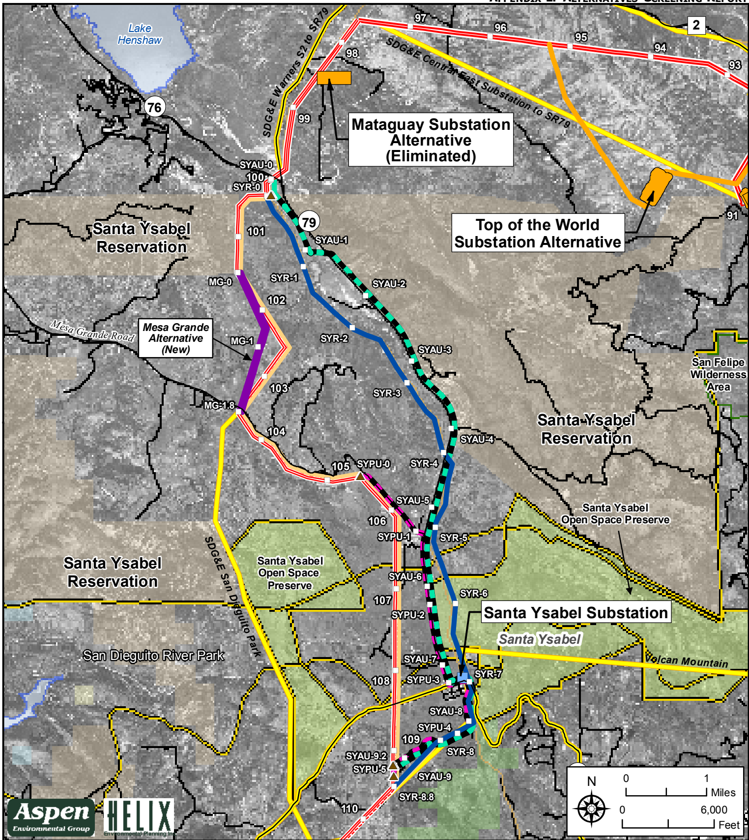
Sunrise Powerlink Project Figure Ap. 1-11 Central Link Alternatives Considered - Santa Ysabel Detail
