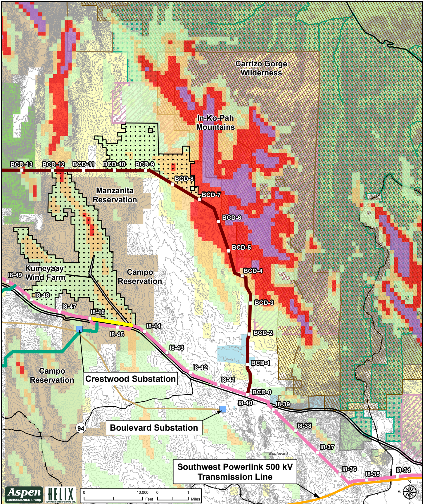
Sunrise Powerlink Project Figure Ap.1-33c New In-Area Renewable Generation Alternative, Wind Component
