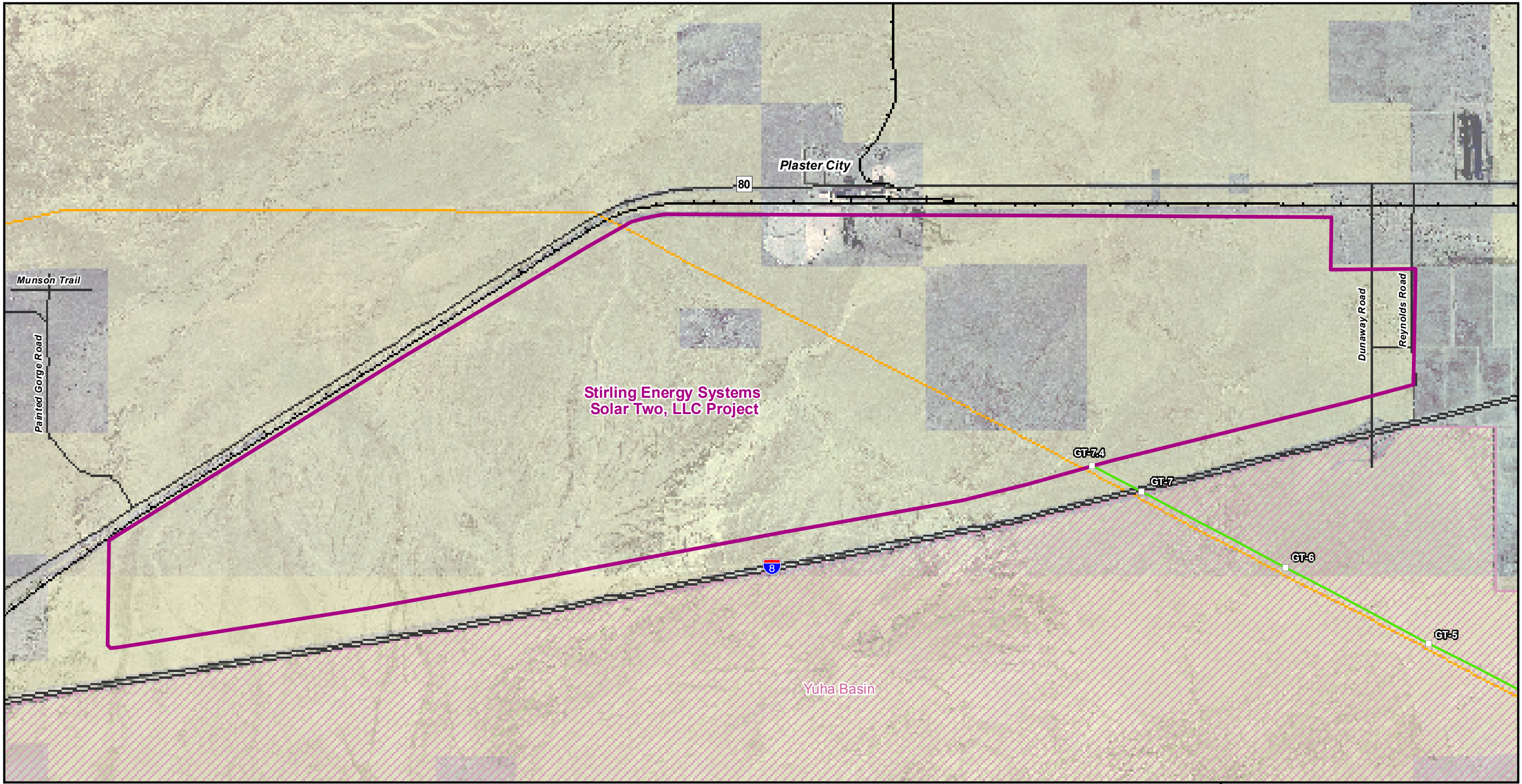
Sunrise Powerlink Project Figure B-44b Connected Actions: Stirling Energy Systems Solar Two Project Site
