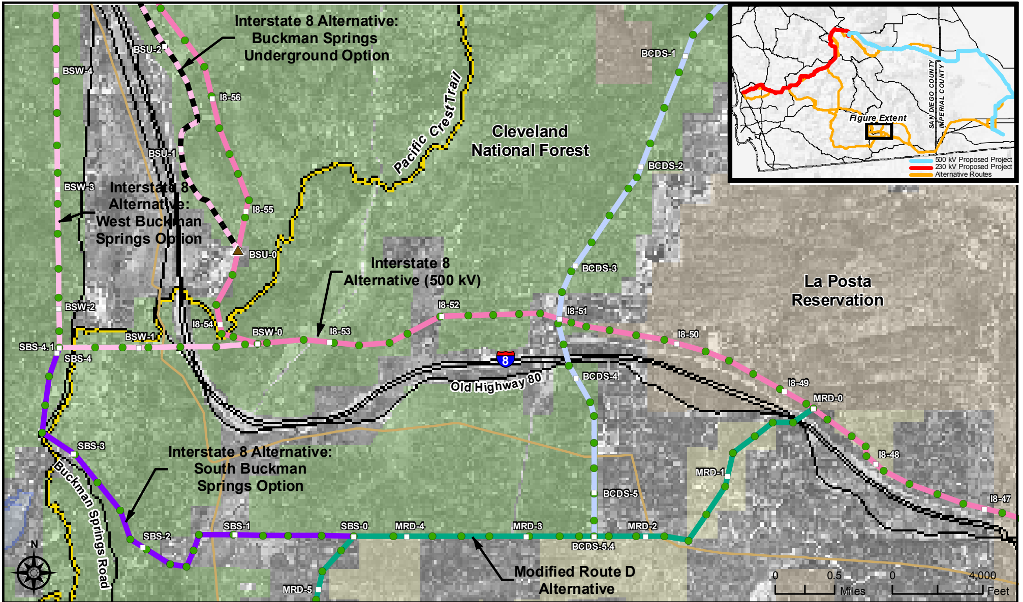
Sunrise Powerlink Project Figure E.1.1-4c Interstate 8 Alternative: South Buckman Springs Option
