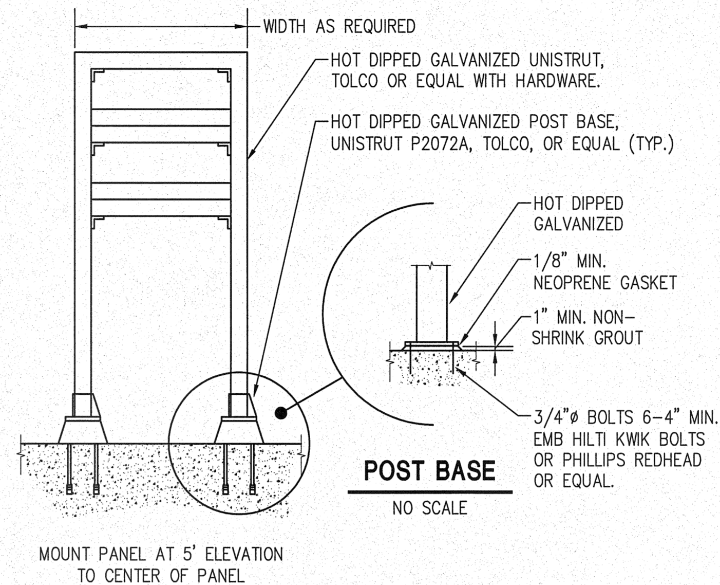
CONTROL PANEL RACK DETAIL NO SCALE
