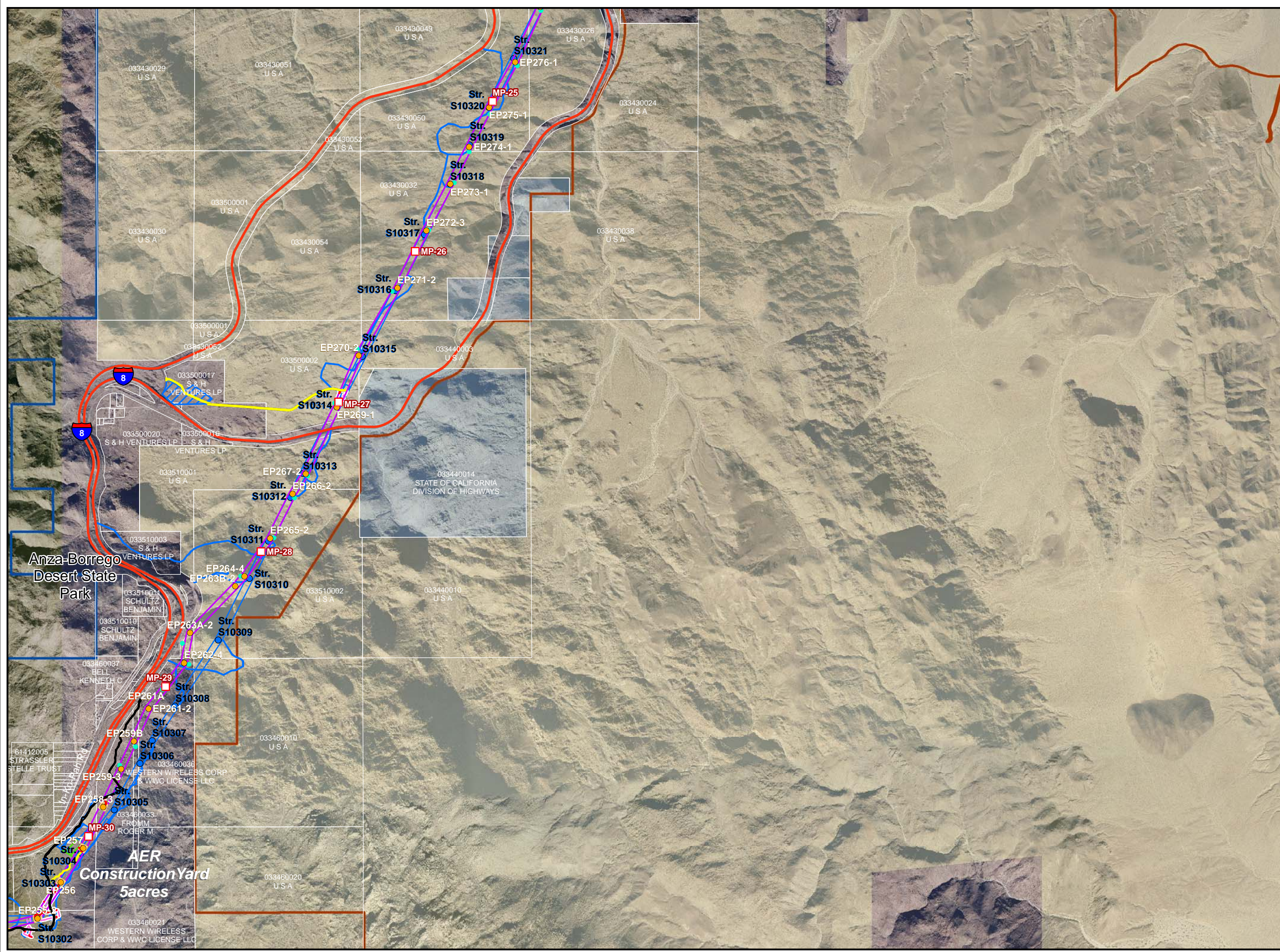
Figure 6 STRUCTURES EP255-2 TO EP276-1
