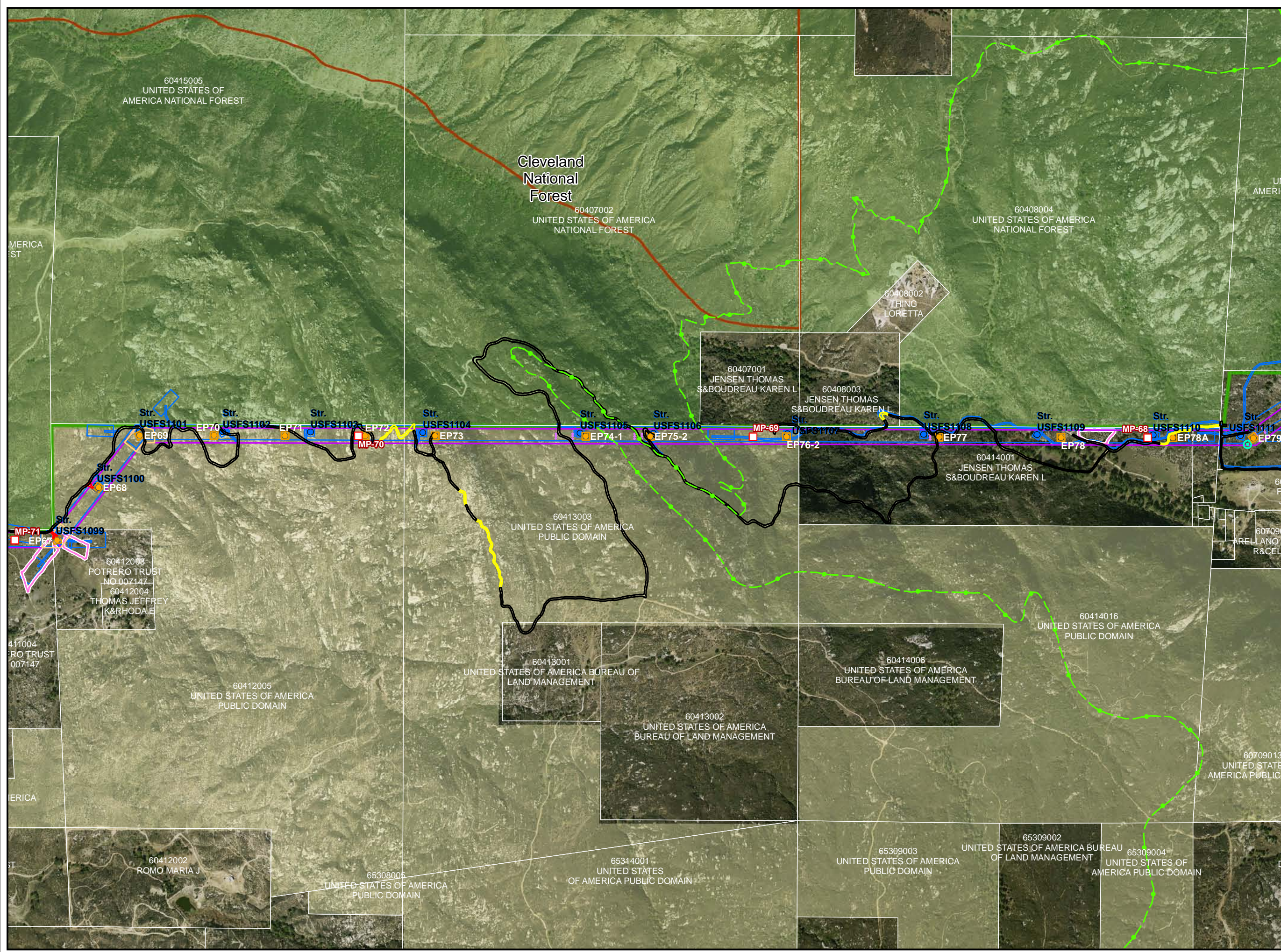
Figure 21 STRUCTURES EP79 TO EP67 (PACIFIC CREST TRAIL)
