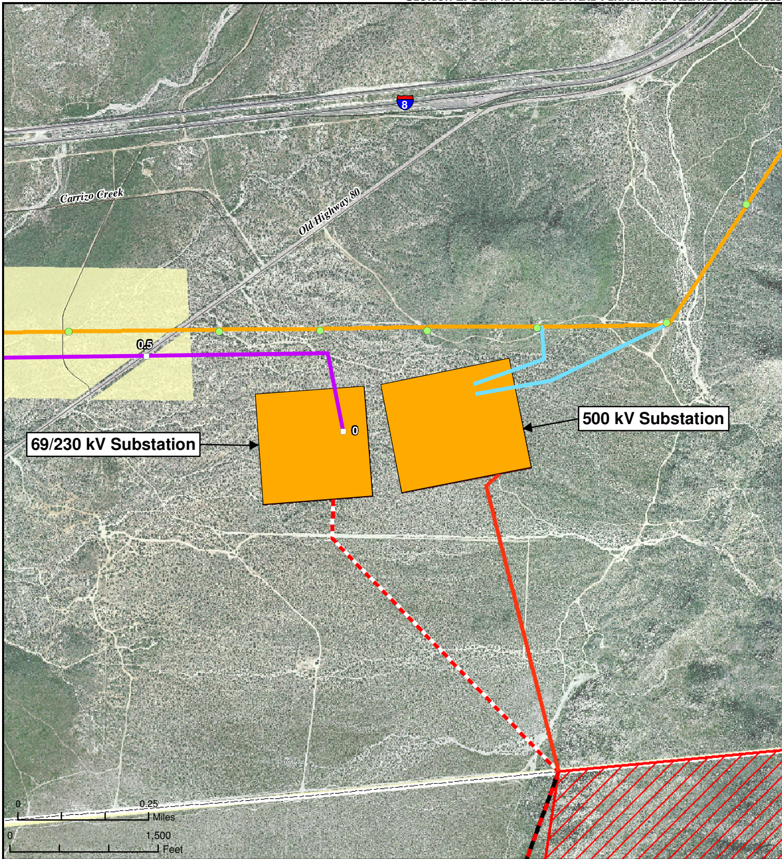
Sunrise Powerlink Project Figure 2-2 Revised SDG&E Jacumba Substation
