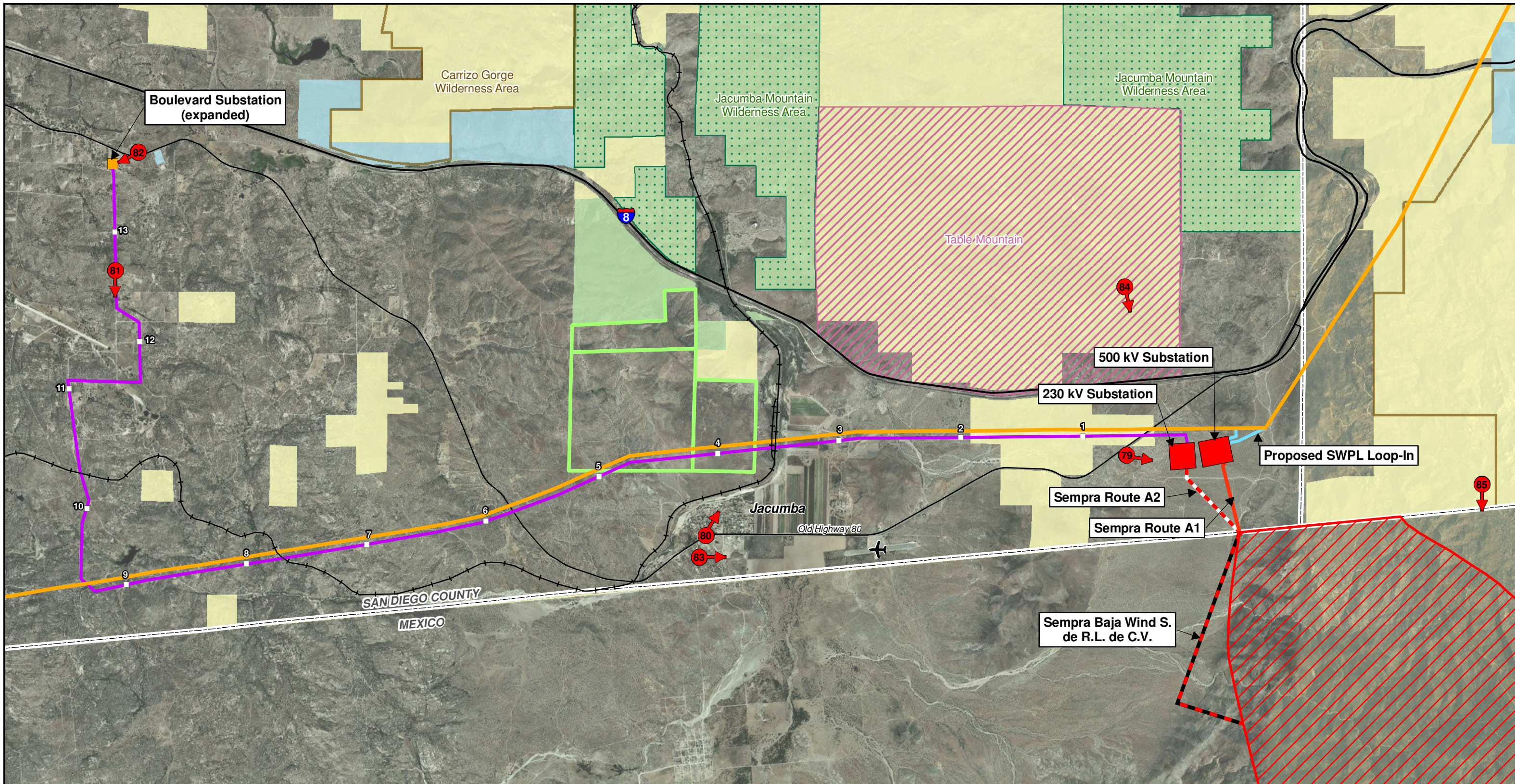
Sunrise Powerlink Project Figure 2.3-1 Sempra Presidential Permit SDG&E 69 kV Transmission Line Key Viewpoints
