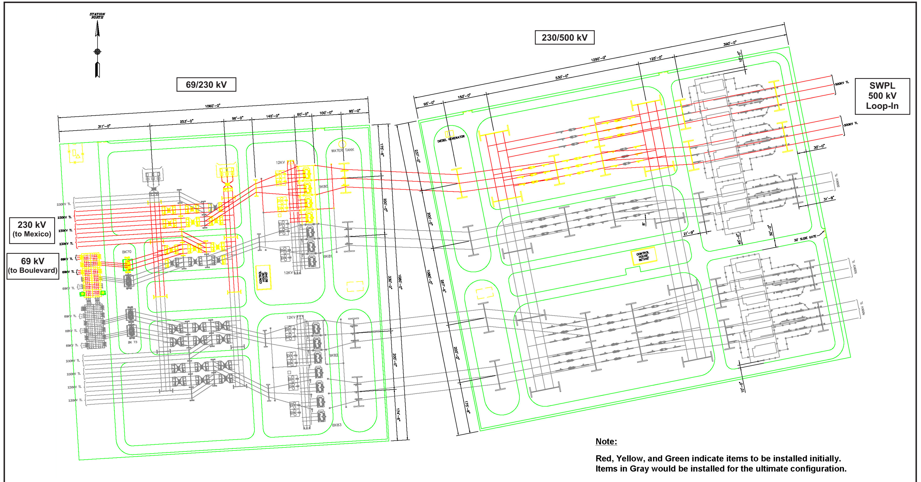
Sunrise Powerlink Project Figure 2-5 Jacumba Substation: Preliminary General Arrangement
