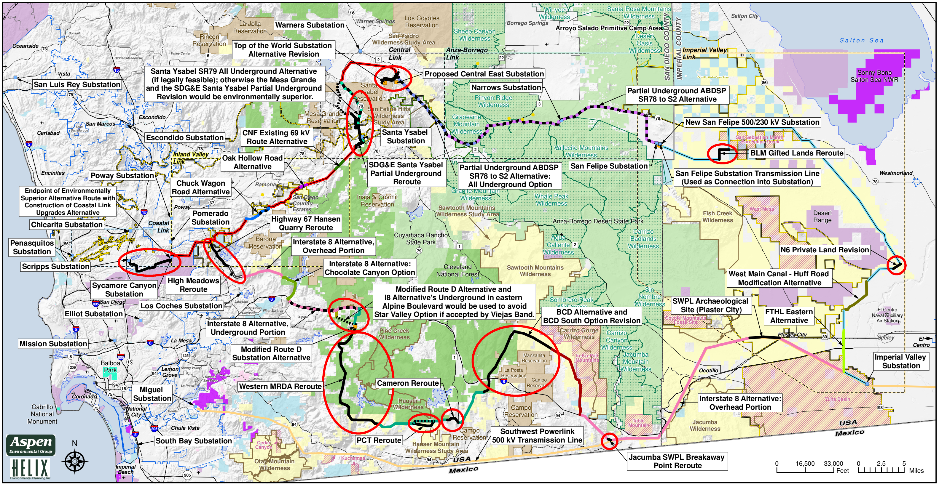
Sunrise Powerlink Project Figure 2 Environmentally Superior Northern Alternative and Modified Environmentally Superior Southern Alternative
