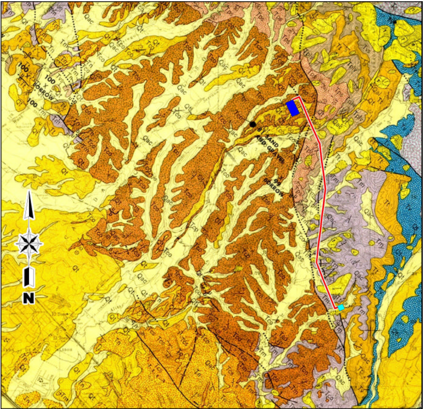
Figure 4. Paleontological Sensitivity, Route 1A
