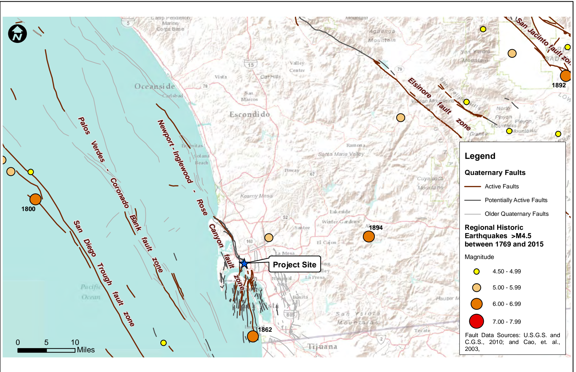
Figure B.3.6-1 Regional Active Faults and Historic Earthquakes
