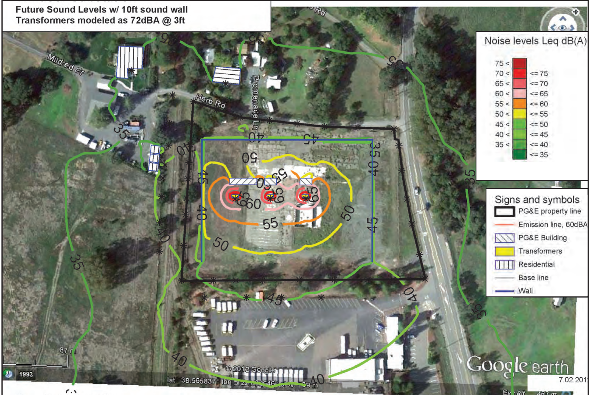
Figure 5.12-2 Transformer Sound Model Plot
