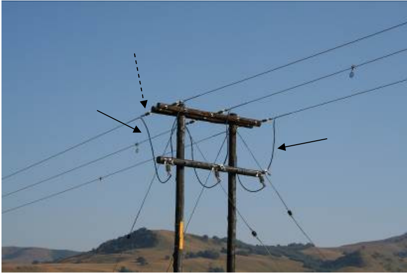
Figure 8. A safe strain pole structure, with insulated jumper wires (black arrows) and sufficiently long insulators (broken arrow) (Photo: EWT-WEP).
