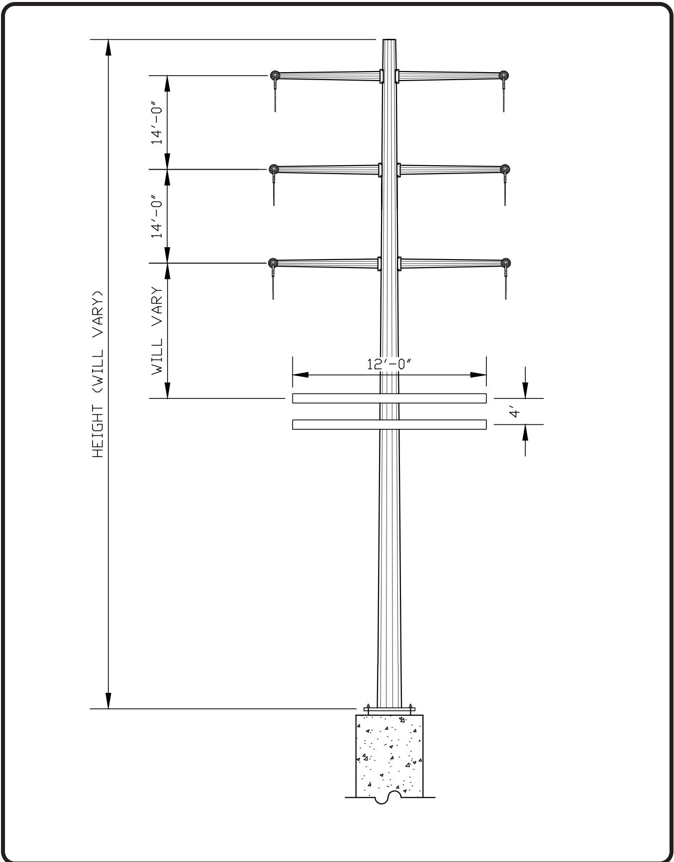
Proposed Double-Circuit Transmission Angle Pole
